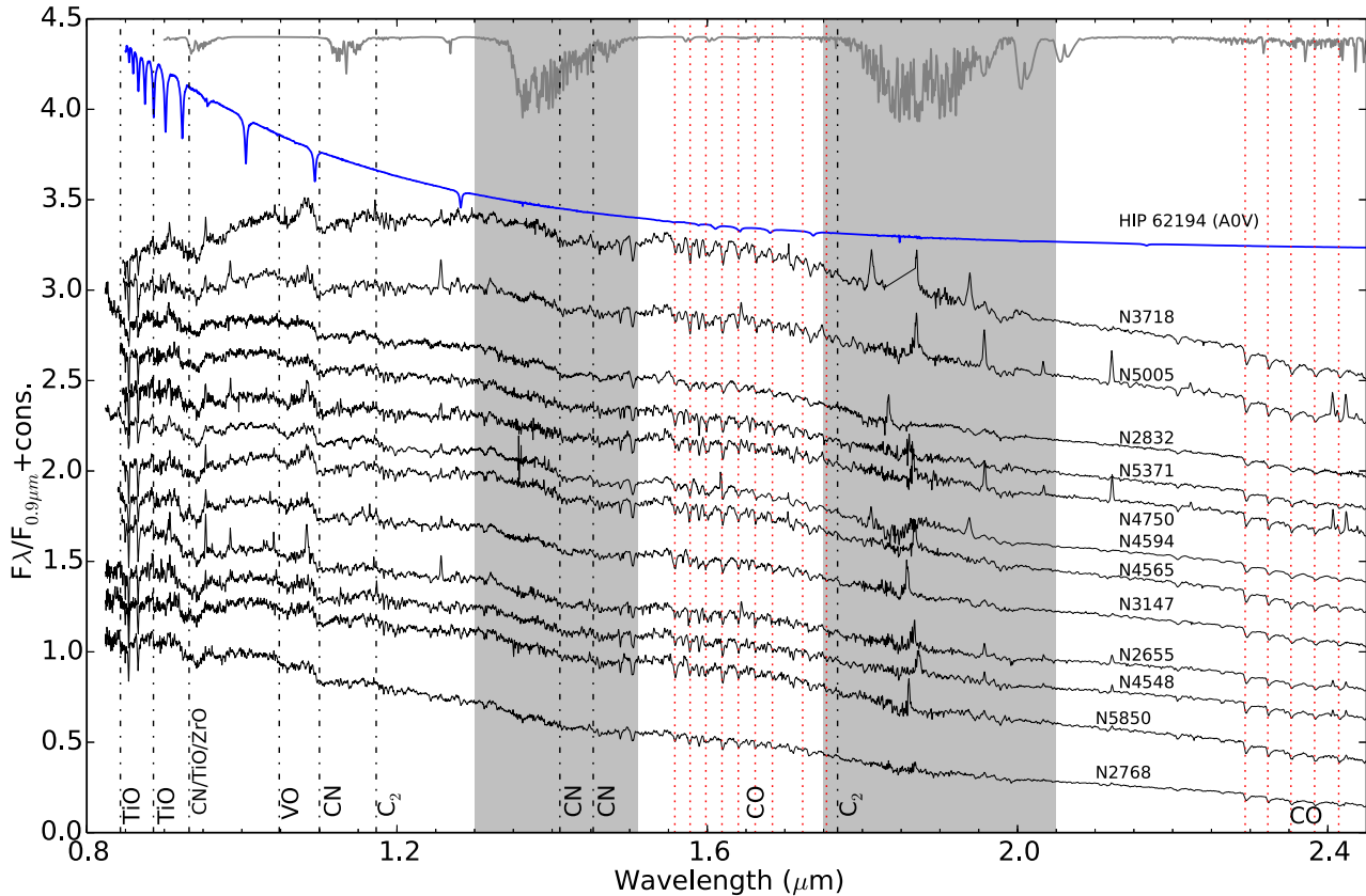
Figure 1. Rest frame spectra of the galaxy sample. Shaded regions indicate broad, stellar H 2 O molecular bands, while dotted lines denote the CO bands. Other molecular bands are labelled at the bottom of the figure. A Mauna Kea atmospheric transmission spectrum for 1 mm H 2 O and 1 airmass is also shown (grey), along with the spectrum of an A0 star (blue) reduced in the same manner as the galaxy data. Because of the small redshifts of the galaxies, the telluric features/residuals in the A0 star and atmospheric spectra do not correspond precisely to those in the galaxy data.
