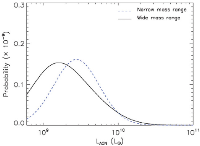
Figure 5. Comparison of the AGN luminosity probability distribution for two different host galaxy mass distributions. The blue dashed line represents the probability distribution for the case where the stellar masses all lie within a narrow range. The black line represents the distribution for the case where the stellar masses are spread over a range of a factor of 10. For programs that detect only a small fraction of the sample (e.g., for L_{\text{AGN}} > 10^{10} L_{\odot} in this example), the detection rate can be much higher for the case where the masses are more widely spread.
