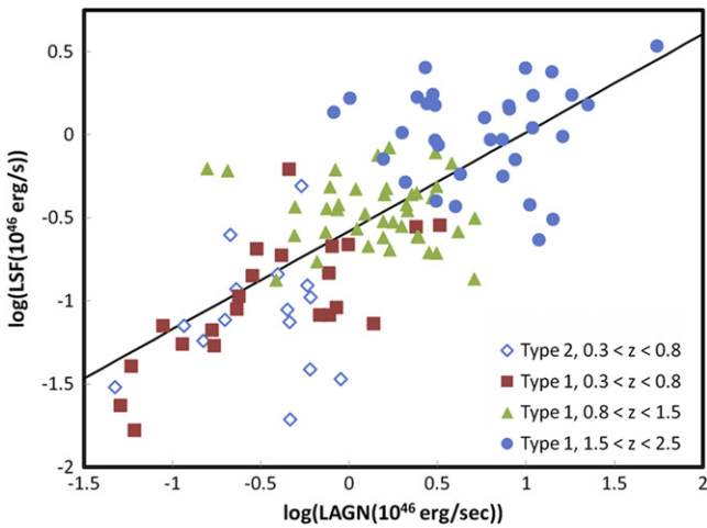
Figure 4. Relation between the IR luminosity of the star formation component and the AGN total luminosity. The solid line is the best-fitting unweighted relationship for all Herschel -detected Type 1 AGN plus the Comparison Sample of Type 2 AGN (selected to have nuclear properties similar to those of the type 1 sources). The fit has a slope of 0.59.
