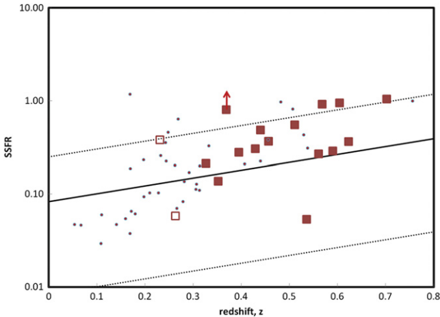
Figure 2. sSFR vs. redshift for the Herschel -detected Type-2 AGNs. The solid line is the sSFR of main sequence galaxies (Elbaz et al. 2011). The dotted lines are a factor of 3 above or 10 below the sSFR of main sequence galaxies, respectively. The filled boxes are for our Comparison Sample, while the unfilled boxes are the two sources with similar AGN properties but at z < 0.3 . The small dots are for the remainder of the Herschel -detected Type-2 galaxies. The lower limit is for J101805.93+385755.8, which is undergoing a strong starburst and for which our mass estimate is an upper limit.
