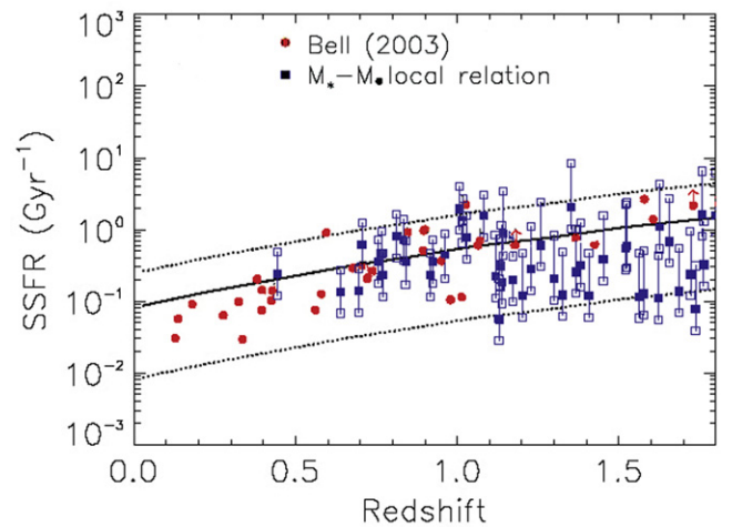
Figure 1. sSFR vs. z for Herschel -detected Type-1 AGNs. The solid line is the sSFR of main sequence galaxies (Elbaz et al. 2011). The dotted lines are a factor of 3 above or 10 below the sSFR of main sequence galaxies, respectively. The filled red circles represent sources with stellar mass estimated by K-band luminosity. The filled blue squares are represent sources with stellar mass estimated from the local mass ratio M_*/M_{\odot} = 700 . The lower open squares are the sSFR values using masses a factor of two lower than the local mass ratio, representing the 1\sigma scatter in the M_*/M_{\odot} relation. The upper open squares are show the upper rms scatter for z < 1.1 but above that value are a factor of 4 above the nominal estimates, allowing for an additional possible factor of 2 systematic error in the M_* estimates due to possible evolution and/or selection of the galaxies on the basis of exceptionally luminous AGNs.
