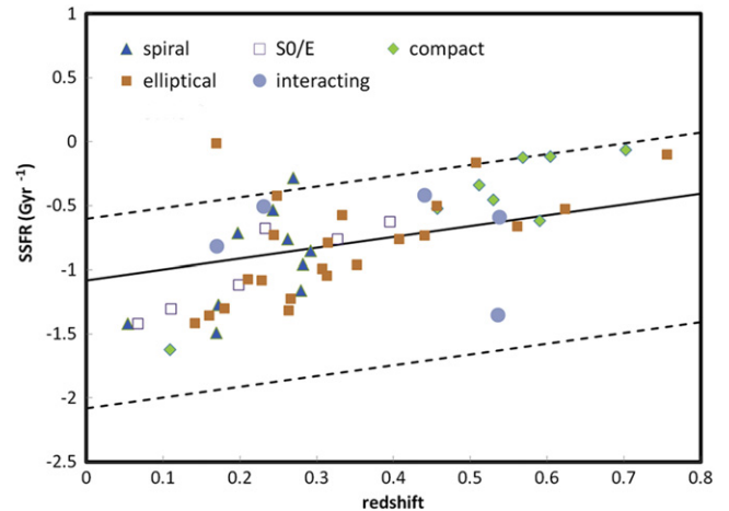
Figure 3. sSFR vs. redshift for Herschel -detected Type-2 AGNs with valid morphology classifications. The solid line is the sSFR of main sequence galaxies (Elbaz et al. 2011). The dotted lines are a factor of 3 above or 10 below the sSFR of main sequence galaxies, respectively. Different symbols represent different galaxy types.
