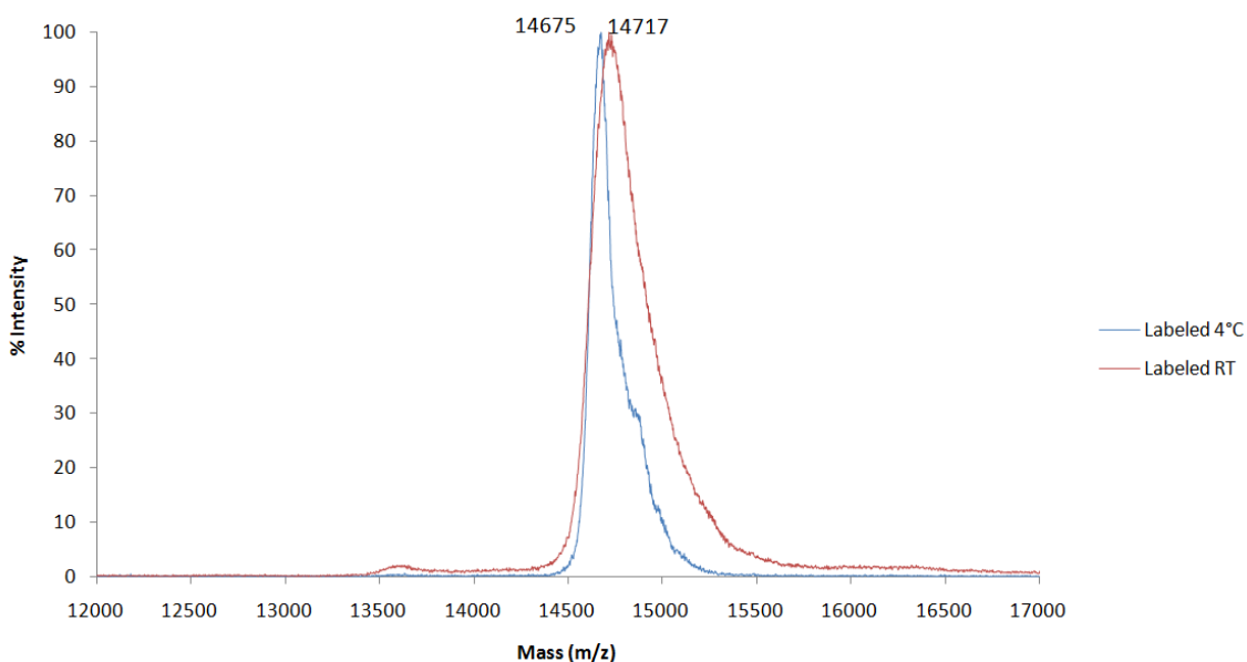
Figure 21: MALDI-TOF mass spectra of ^{15}\text{N} labeled wt-TTR purified at RT or 4^\circ\text{C} . Spectra with a range from 12000 to 17000 m/z of ^{15}\text{N} labeled recombinant wt-TTR purified and stored either at RT (red) or 4^\circ\text{C} (blue). Peaks for the 4^\circ\text{C} and RT samples were 14675 and 14717 Da, respectively.
