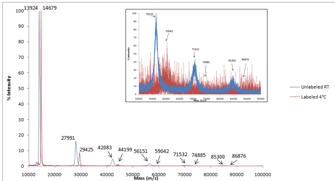
Figure 24: Overlay of MALDI-TOF mass spectra of unlabeled wt-TTR gel filtered at RT and ^{15}\text{N} labeled wt-TTR at 4^\circ\text{C} showing multimers formed during analysis. Spectra with a range from 10000 to 100000 m/z of unlabeled recombinant wt-TTR gel filtered at RT (blue) and ^{15}\text{N} labeled at 4^\circ\text{C} . Up to 6 monomers containing multimers are shown. The insert shows the same spectra with percent intensity relative to the most intense peak, with a range from 50000 to 95000 m/z.
