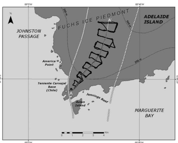
Fig. 2. Measured tracks in November and December 2002. GPS and RES data in black lines and ATM data in white circles. The location of the topographic profile A–A' (white crosses) shown in Figure 4 is included. The contour lines were extracted from BAS (2001).
