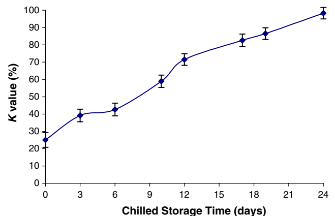
Fig. 2. K value (%) assessment (Bars denote standard deviation of the mean ( n = 5 )) in Coho salmon muscle during chilled storage.
