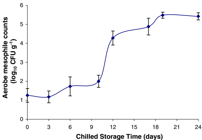
Fig. 3. Evolution of total aerobic mesophile growth ( \log_{10} \text{CFU g}^{-1} fish muscle) (Bars denote standard deviation of the mean ( n = 5 )) in Coho salmon muscle during chilled storage.
