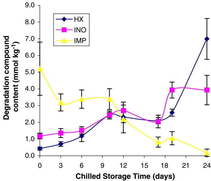
Fig. 1. Evolution of inosine 5'-monophosphate (IMP), inosine (INO) and hypoxanthine (HX) contents (mmol kg -1 fish muscle) (Bars denote standard deviation of the mean ( n = 5 )) in Coho salmon muscle during chilled storage.
