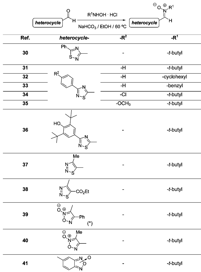
Scheme 3. Synthesis and Structure of New Heteroarylnitrones a
