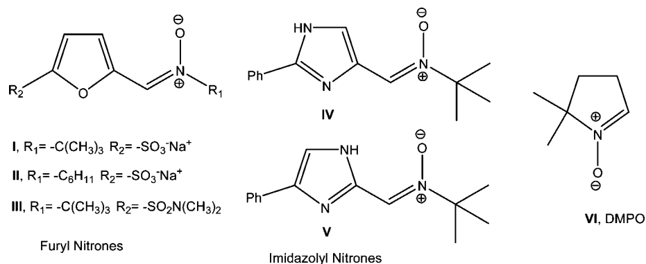
Figure 2. Heteroaryl nitrones with neuroprotective and spin trapping properties.
