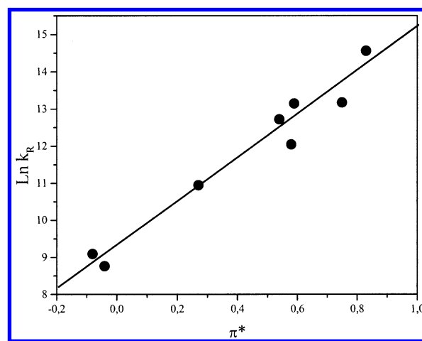
FIGURE 3. Dependence of the chemical reaction rate constant, k_R , for reaction of DMD with singlet oxygen on the solvatochromic parameter \pi^* .
