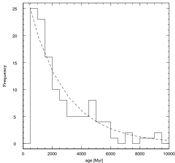
Figure 18. Age distribution of known open clusters older than 500 Myr. The dashed exponential line has an e-folding time of 2 Gyr.
