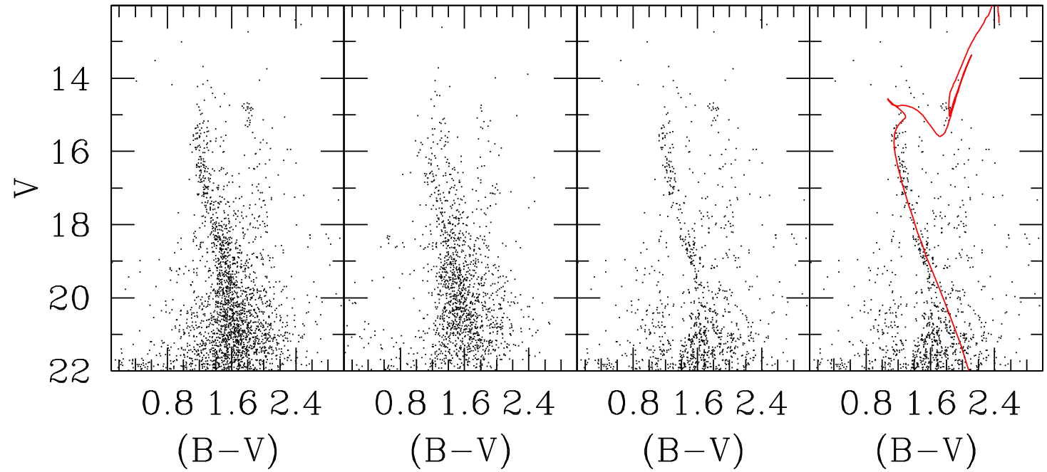
Figure 15. Left panel: CMD of Skiff 1; Mid-left panel: CMD of the control field; Mid-right panel: the clean CMD; Right panel: Isochrone solution for Skiff 1: the 1.2 Gyr isochrone is shifted by E(B-V) = 0.85 en V-M_V = 13.70
