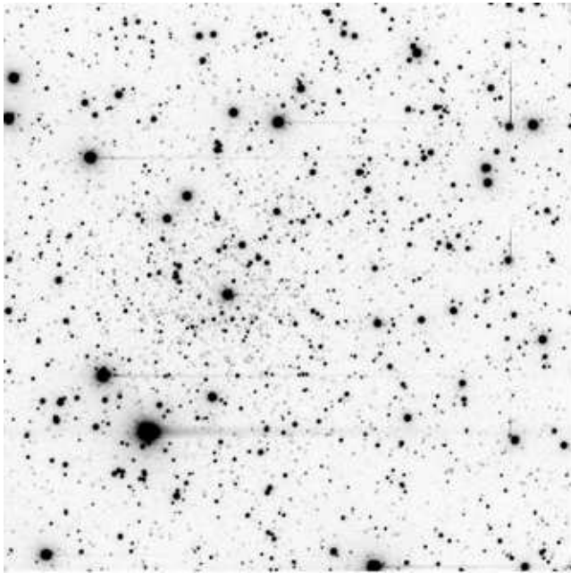
Figure 4. V 60 secs image centered on Berkeley 56. North is up, east on the left.
