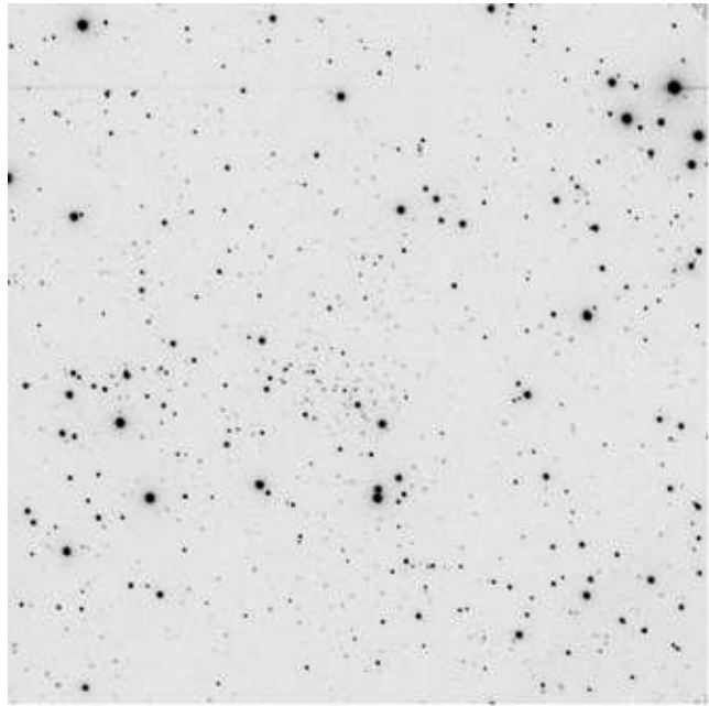
Figure 6. V 60 secs image centered on Berkeley 5. North is up, east on the left.
