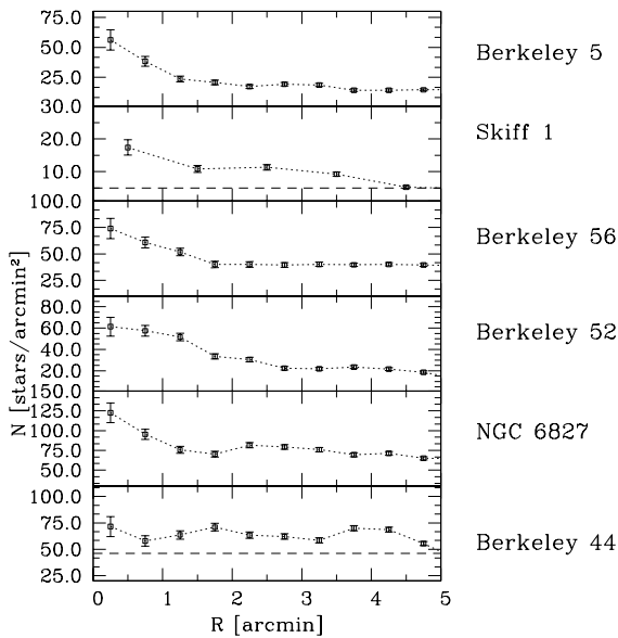
Figure 7. Star counts in the V passband for the clusters under investigation. The dashed lines in the Berkeley 44 and Skiff 1 panels indicate the level of the background as derived from the accompanying control field.
