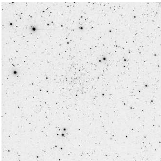
Figure 3. V 60 secs image centered on Berkeley 52. North is up, east on the left.
