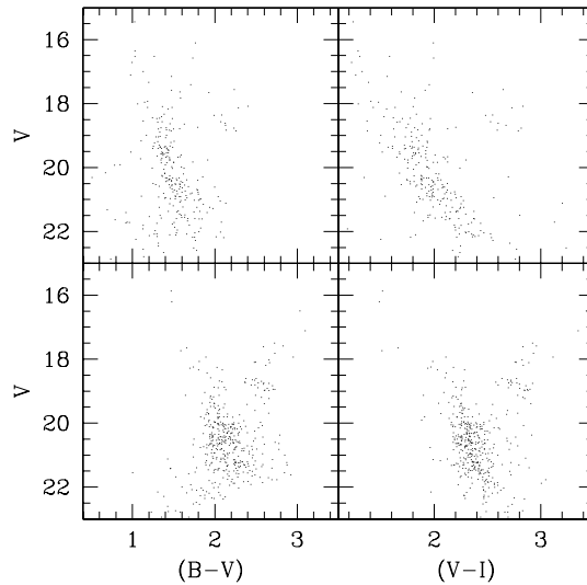
Figure 9. Color Magnitude Diagrams of Berkeley 52 (lower panels) and Berkeley 5 (upper panels). Only the stars inside the cluster radius are shown.
