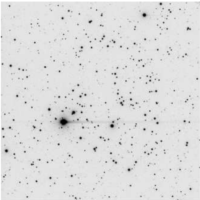
Figure 5. V 60 secs image centered on Skiff 1. North is up, east on the left.
