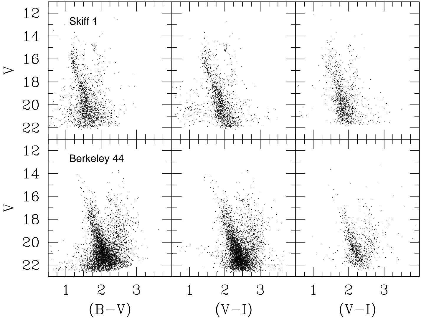
Figure 10. Color Magnitude Diagrams of Skiff 1 and Berkeley 44. The right panels are the comparison field. Note the anomalous blue MS with a TO at V = 19.5 in the CMD of Skiff 1 and its control field.
