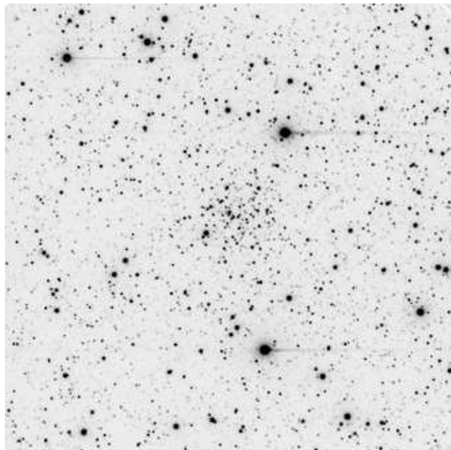
Figure 2. V 60 secs image centered on NGC 6827. North is up, east on the left.
