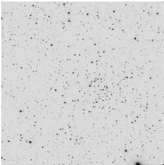
Figure 1. V 60 secs image centered on Berkeley 44. North is up, east on the left. The field is 10 arcmin on a side.
