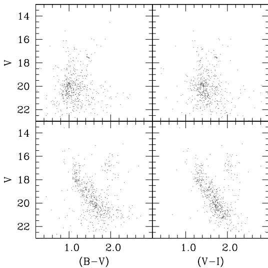
Figure 8. Color Magnitude Diagrams of NGC 6827 (lower panels) and Berkeley 56 (upper panels). Only the stars inside the cluster radius are shown.
