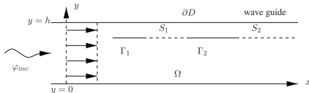
Fig. 11. Geometry of the two plates problem.
