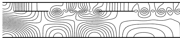
Fig. 13. Real part of the total velocity potential for two plates L = 4 , k = 1 and M = 0.3 . 21 isolines between -1 and 1 . F_1 = 0.49 + 0.05i and F_2 = 0.24 - 0.48i . |F_1| = 0.49 and |F_2| = 0.54 .
