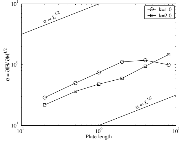
Fig. 8. Parameter \alpha = \partial|F|/\partial\sqrt{M} versus the plate length, for the frequencies k = 1 and k = 2 .
