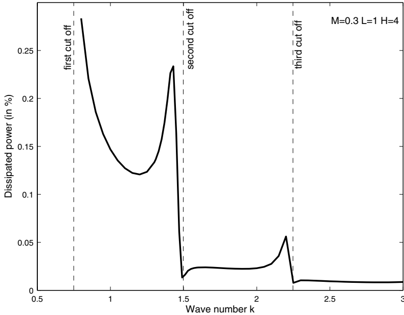
Fig. 10. \Pi_D/\Pi_0 versus k for M = 0.3 and L = 1 .
