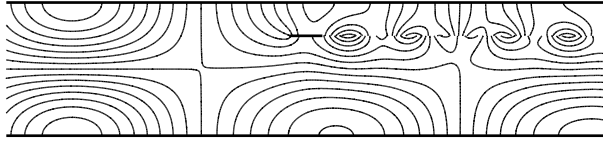
Fig. 6. Real part of the total velocity potential for a Mach number M = 0.3 , k = 1 and with a plate length L = 1 (15 isolines from -0.9 to 0.9 ).
