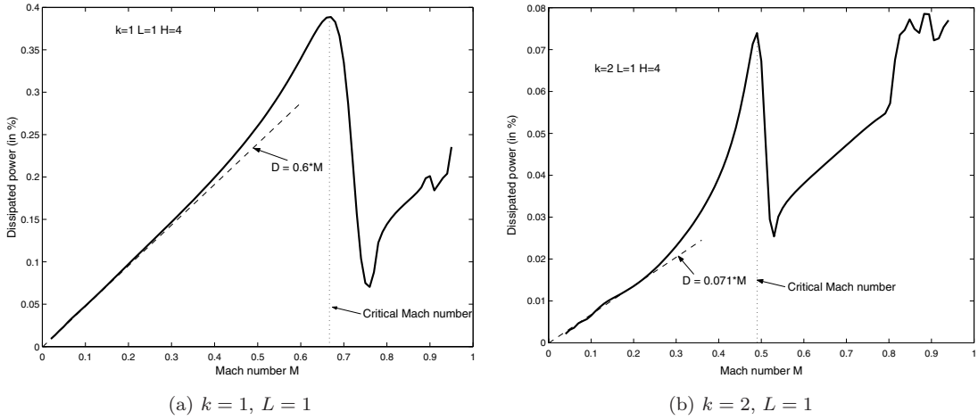
Fig. 9. \Pi_D/\Pi_0 versus M .
