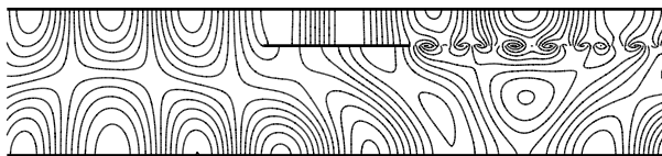
Fig. 5. Real part of the total velocity potential for a Mach number M = 0.3 and with a plate length L = 4 (15 isolines from -0.7 to 0.7 ). The incident wave, of acoustic wavenumber k = 2 , corresponds to the first antisymmetric guided mode.
