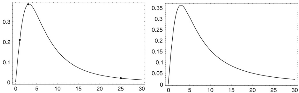
Fig. 7. Plot of the efficiency E as a function of \omega in the sinusoidal case (left) and in the smooth sawtooth potential case (right). We observe that in both cases, the maximum is extremely well defined. Dots (left) correspond (\omega, E(\omega)) taking the values (1, 0.210) , (3, 0.385) , (25, 0.021) and will be reused in Fig. 8.
