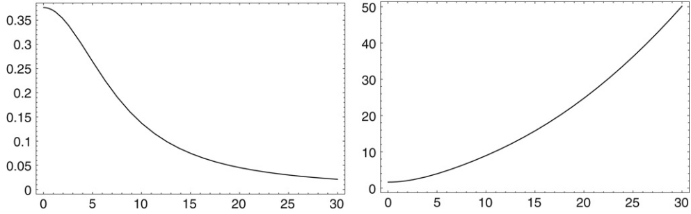
Fig. 9. Plot of the mobility \mu_\omega (left) and the effective temperature \Theta (measured in units of 1/k_B ) of the tilted Brownian ratchet for values of \omega ranging between 0 and 30 in the sinusoidal case.
