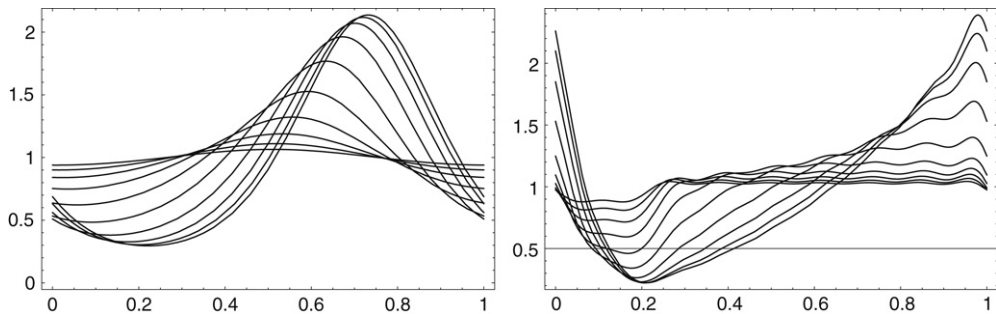
Fig. 10. Plot of the stationary solution g_\omega of the tilted Brownian ratchet for increasing values of \omega ranging between 1 and 100 (logarithmic scale) in the sinusoidal case (left) and in the smooth sawtooth potential case (right).
