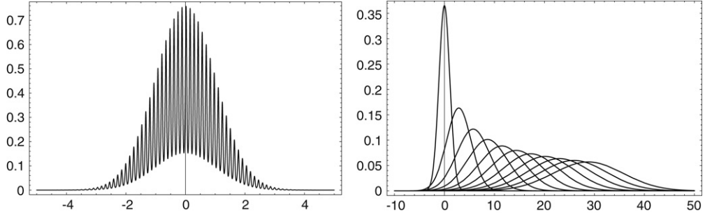
Fig. 3. In the sinusoidal case, the limiting function u_{\infty} is shown on the left, in self-similar-variables, while on the right, the diffuse, travelling front F_{\infty} is plotted in the original variables for t = 0, 1, \dots, 20 . Here we take \omega = 5 and (left) u_{\infty}(t, x) is shown as a function of x for t = 2 .
