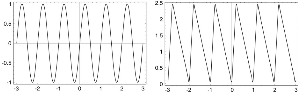
Fig. 1. Plots of the potential \psi in the sinusoidal case (left) and in the asymmetric smooth sawtooth potential (right), which is computed here as a truncated Fourier series of x \mapsto x/x_0 if x < x_0 and x \mapsto (1-x)/(1-x_0) if x > x_0 , with x_0 = 0.2 .
