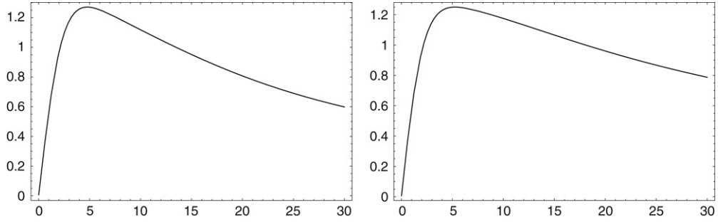
Fig. 5. Plot of the Péclet number Pe as a function of \omega in the sinusoidal case (left) and in the smooth sawtooth potential case (right).
