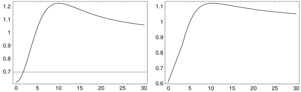
Fig. 4. Plot of the diffusion coefficient \kappa_{\omega} as a function of \omega in the sinusoidal case (left) and in the smooth sawtooth potential case (right).
