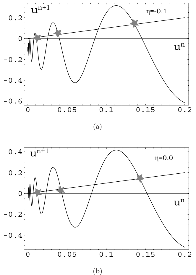
Fig. 5. Schematic representation of the first return map (6) for different values of \eta : (a) \eta = -0.1 , and (b) \eta = 0.0 . The stars stand for the equilibria points.
