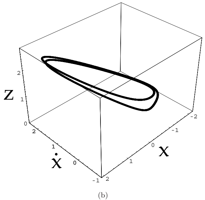
Fig. 3. Limit cycle solution exhibits by model (4) by \beta = -0.814 , \delta = 1.0 , \mu = 0.6 , (a) \nu = 0.31 , and (b) \nu = 0.295 .
