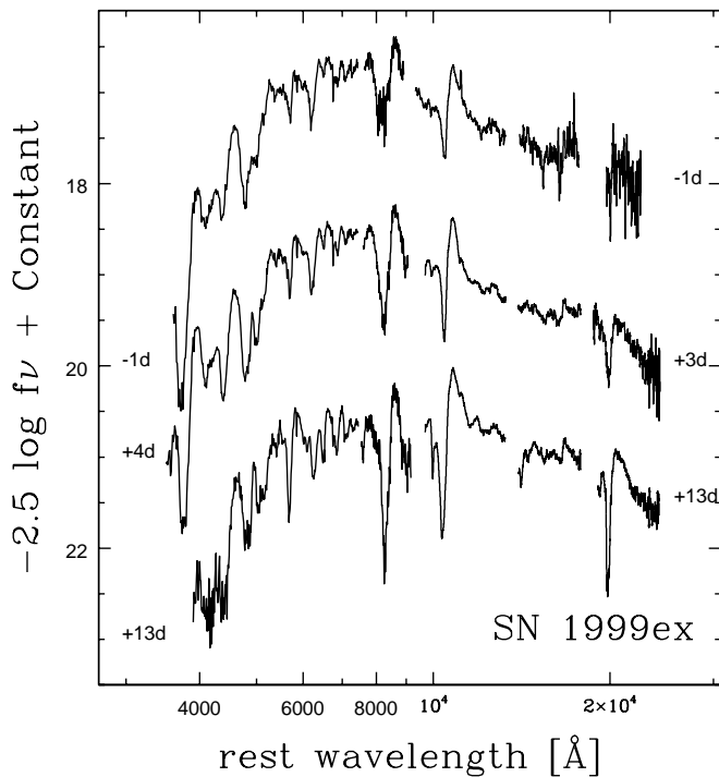
FIG. 12.—Combined optical and IR spectra of SN 1999ex in AB magnitudes. Days since B maximum are indicated next to each spectrum.
