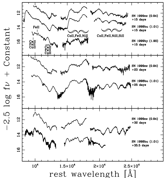
FIG. 8.—Comparison of the postmaximum IR spectra of SNe 1998bu, 1999by, and 1999ee. Time (in days) since B maximum is indicated for each spectrum, along with the decline rates \Delta m_{15}(B) .
