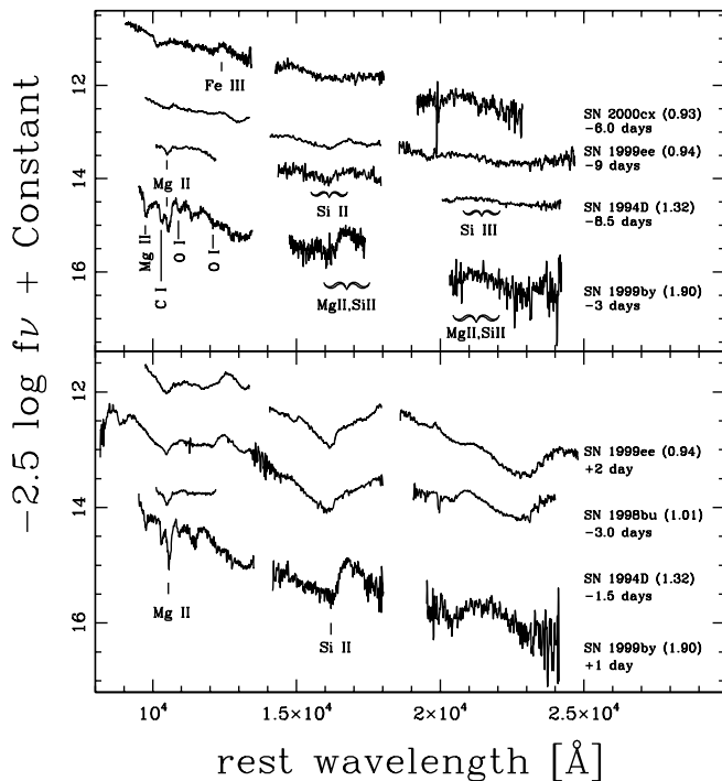
FIG. 7.—Comparison of the premaximum and maximum-light IR spectra of SNe 1994D, 1998bu, 1999by, 1999ee, and 2000cx. Time (in days) since B maximum is indicated for each spectrum, along with the decline rates \Delta m_{15}(B) .
