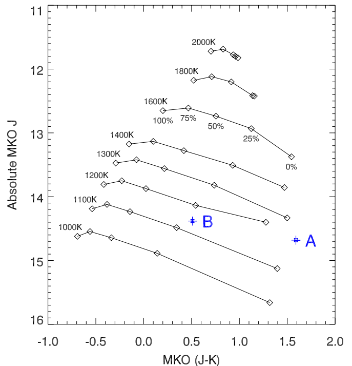
Figure 10. Absolute MKO J magnitude as a function of MKO J-K for the partly cloudy models of Marley et al. (2010) with cloud hole fractions of 0%, 25%, 50%, 75%, and 100%. The atmosphere models have effective temperatures 1000–2000 K and use equilibrium chemistry with f_{\text{sed}} = 2 and \log g = 5 . WISE 0611–0410 A has properties consistent with a fully cloudy atmosphere. WISE 0611–0410 B is most closely matched to a model with T_{\text{eff}} = 1150 K and 25% fractional hole coverage.
