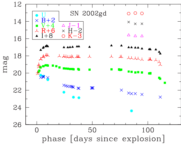
Figure 5. Early-time UBVRJIHK light curves of SN 2002gd.
