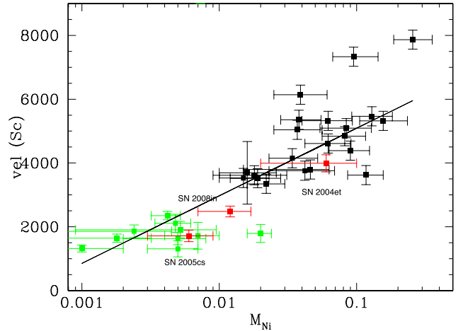
Figure 17. Ejecta velocities versus ^{56}\text{Ni} masses. The expansion velocities are obtained from measuring the position of the minimum of the \text{Sc II } \lambda 6246 \text{ \AA} line. Symbols are as in Fig. 16.
