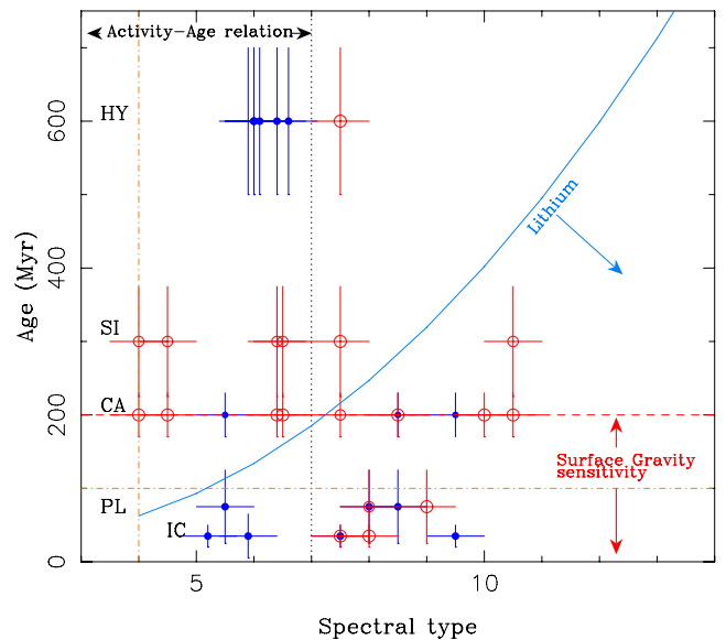
Figure 6. This figure (updated fig. 9 from Paper I) illustrates how an object would be selected for the various methods of age constraining. Candidates that appear to the right of the lithium edge (blue continuous line) can be followed up with a lithium test programme. Objects that appear younger than 200 Myr (horizontal red dashed line) are eligible for follow-up using spectroscopic gravity-sensitive features. Vertical and horizontal orange dot-dashed line represents the Schlieder et al. (2012) limits for the \text{Na I} diagnostic applicability. We here took into account the 200 Myr limit. Candidates that fall to the left of the spectral type = M7 limit (vertical black dotted line) would thus be suitable for age/activity relation follow-up, although candidates with a spectral type close to M7 may be subject to large uncertainties on their age. Some candidates cannot be tested by any of these methods but will be eligible for age testing using v \sin i . Sample A targets are plotted as blue filled circles and sample B as red open circles. We plotted up to two candidatures for targets with multiple MG.
