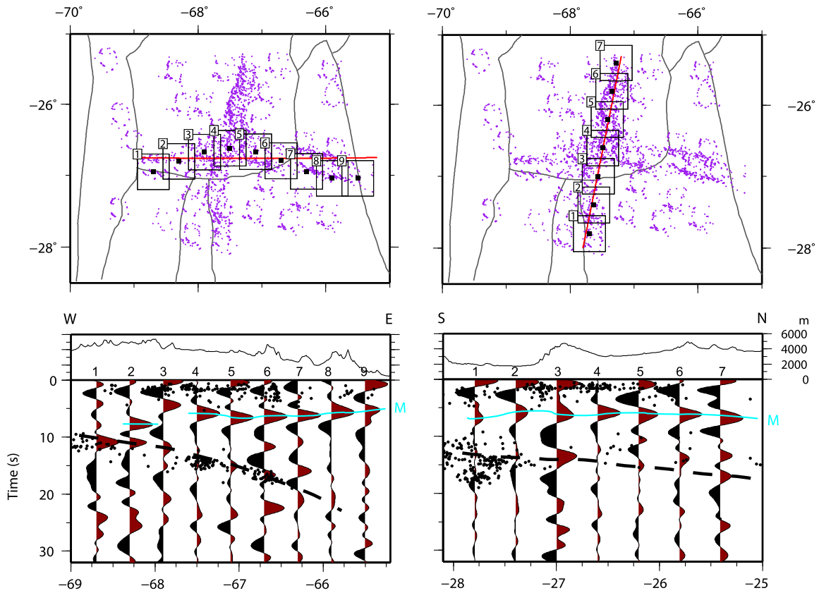
Fig. 3. Upper panels: Map showing the stacking boxes (black squares with bold squares in the center of each box) and piercing points (violet circles) for two orthogonal EW (left) and NS (right) profiles with the highest station density. The piercing points are calculated at a depth of 60 km, roughly representing the depth of the Moho. Receiver functions are stacked for piercing points falling into each box with a size of 0.5^\circ overlapping by 0.1^\circ . Lower panels: Stacked receiver functions along the two profiles. Positive amplitudes are shaded in red, negatives in black. Topography is sampled every 1 km across the red line on the maps. Black dots on the profiles are hypocenters from Mulcahy et al. (submitted for publication) . The Moho phases are marked by the blue line and indicated as M on the profiles. (For interpretation of the references to color in this figure legend, the reader is referred to the web version of this article.)
