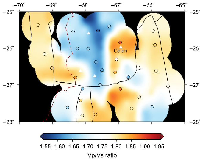
Fig. 6. Map of crustal V_p/V_s ratio determined by the H-K analysis (Zhu and Kanamori, 2000). The Ps Moho conversion and the crustal multiples (PpPs and PpSs) are used to determine the crustal thickness and V_p/V_s ratio. Black lines mark the tectonic units as shown in Fig. 1. The southern Puna is characterized by a low crustal V_p/V_s ratio (<1.70), indicating a felsic crustal composition. The V_p/V_s ratio beneath Cerro Galan is anomalously high (1.87), implying presence of melts. The position of Galan is included as a reference.
