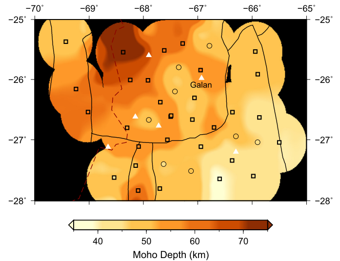
Fig. 7. Map of crustal thickness in the study area. Small circles represent the center of the boxes used to obtain the Moho depth. Most of the values are obtained by the H-K analysis (indicated by bold squares). For some of the boxes where the H-K analysis failed, an average V_p/V_s ratio of 1.74 is used to estimate the Moho depth (indicated by light circles). Black lines mark the tectonic units as in shown Fig. 1. The crust is thicker (>60 km) in the west and northwest beneath the volcanic arc. The Moho in the Puna region is relatively flat with depths varying between 50–60 km. To the southeast, the Sierras Pampeanas have a crustal thickness between 35–45 km. The position of Galan is included as a reference.
