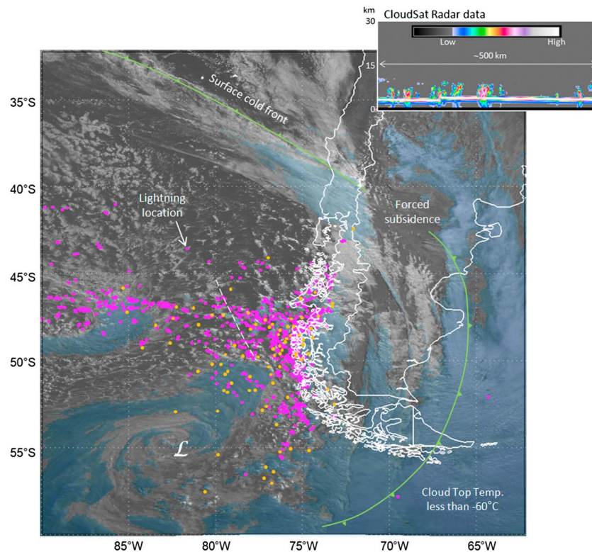
Figure 9. Main panel: Stroke locations from WWLLN (purple circles) and Startnet (orange circles) during the afternoon of April 30, 2012, superimposed on the GOES-13 visible image at 1745 UTC of that day. The faint blue shading indicates cloud top temperatures lower than -60^{\circ}\text{C} derived from the concurrent GOES-13 infrared (IR2) image. Also indicated is the position of a cold front falling in southern Chile. Inset: Quick look image from the CloudSat radar data along the transect in white, dashed line in the main map for 1818 UTC May 1, 2012.
