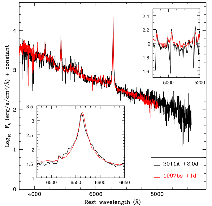
Figure 15. Comparison between the SN 2011A spectrum taken 2.0 days after discovery, in black, and that of SN 1997bs taken on April 16th, one day after discovery, in red (no detection on 1997 April 10th). In the top right inset we zoom on the Fe II lines, \lambda\lambda 4923, 5018, 5169 . In the bottom left inset we zoom on the H \alpha emission line. We applied a total reddening of E(B - V) = 0.24 mag to SN 1997bs in order to match the continua.
