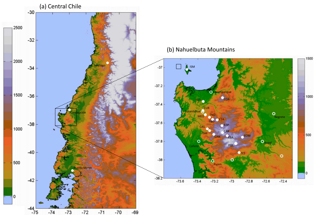
FIG. 1. Topographic maps of (a) south-central Chile and (b) NM area. In (b), filled circles correspond to the location of the AFEX rain gauges (see codes and further details on Table 1) and open circles correspond to the location of meteorological stations from DMC/DGA used in this study. Note that the color scale is different in each map. The small box in (b) near Isla Santa Maria indicates the column in WRF intermediate domain from where we take the wind and thermodynamical profiles to force the LT model.
