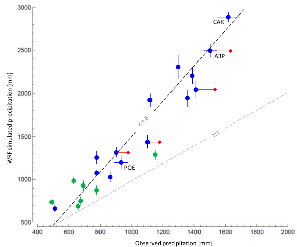
FIG. 6. Scatterplot of observed ( x axis) and WRF-simulated (inner domain, y axis) accumulated precipitation for the winter of 2011 on the AFEX rain gauges (blue circles) and DMC/DGA stations (green circles). The WRF values are obtained by bilinear interpolation of the gridded results to the station location (latitude–longitude). The vertical lines indicate the standard deviation of the WRF results when offsetting such location by \pm 0.1^\circ ( \sim 10 km). The horizontal lines in the three AFEX stations above 1100 m MSL (A3P, PQE, and CAR) are because the full winter precipitation was estimated there on the basis of the rain events only (see appendix B). The red diamonds in four stations in the windward slope of the NM are an upper bound of the observed precipitation considering a 10% wind-induced undercatch. The 1:1 and 1:1.5 lines are shown for reference.
