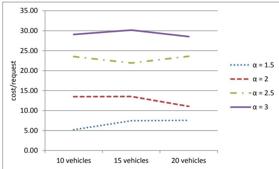
Figure 5.2 Difference in cost/request between Distance-Tabu and Congestion-Tabu
