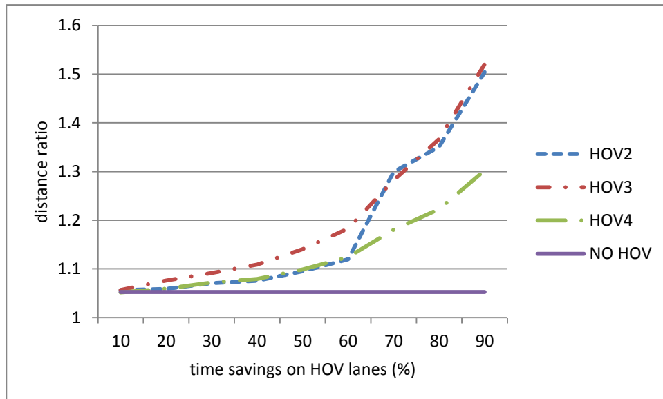
Figure 5.3 Distance Ratio Sensitivity to Time Savings on HOV Lanes
