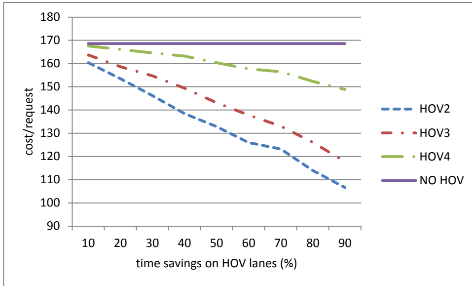
Figure 5.5 Cost/request Sensitivity to Time Savings on HOV Lanes
