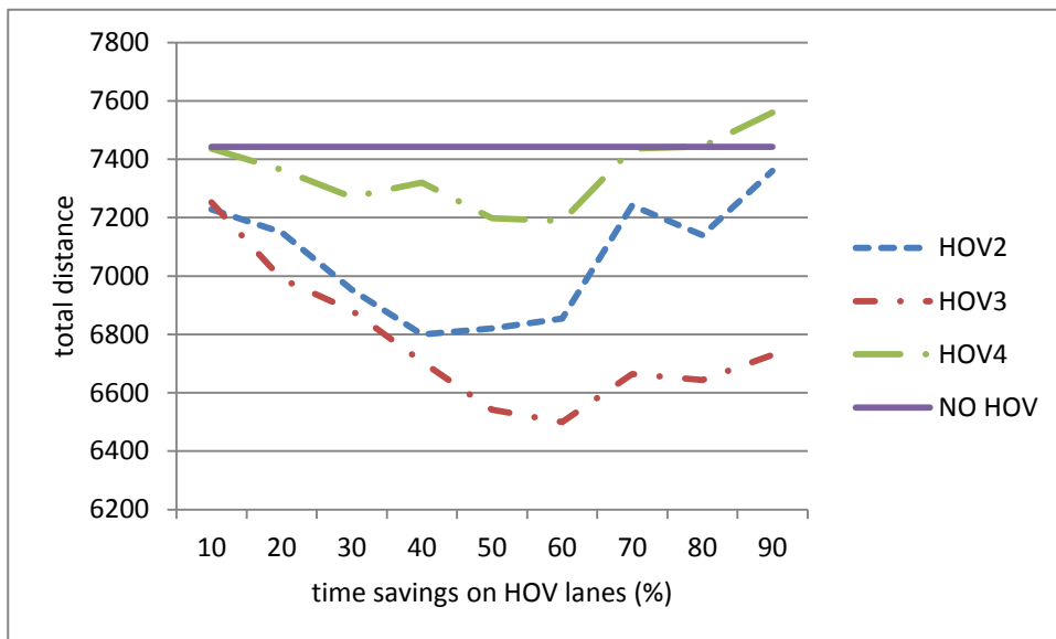
Figure 5.6 Total Distance Sensitivity to Time Savings on HOV Lanes
