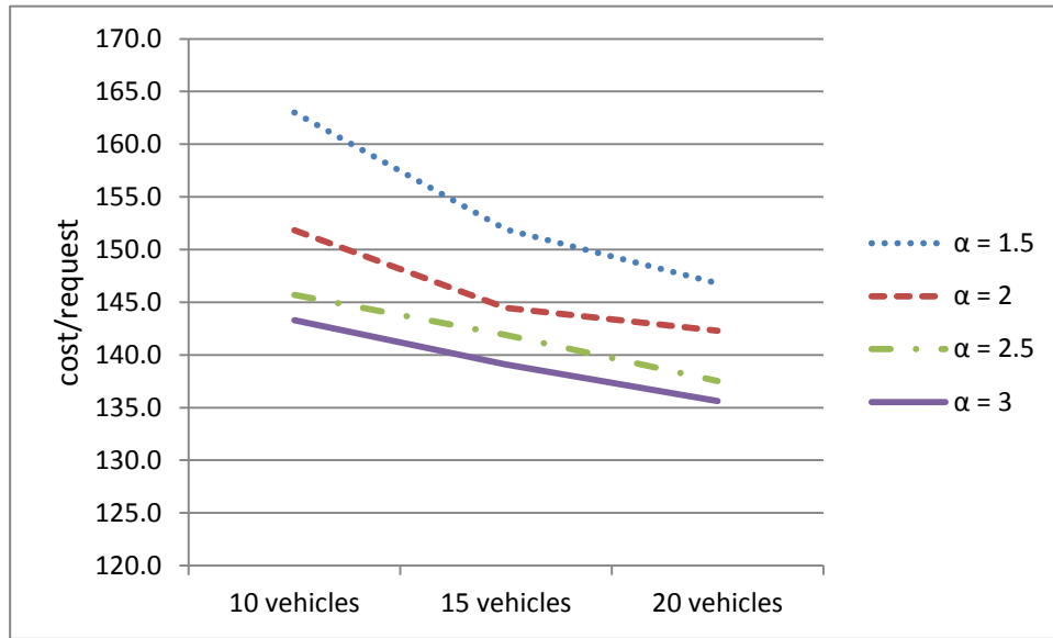
Figure 5.1 Cost/request for Different \alpha 's Using Congestion-Tabu
