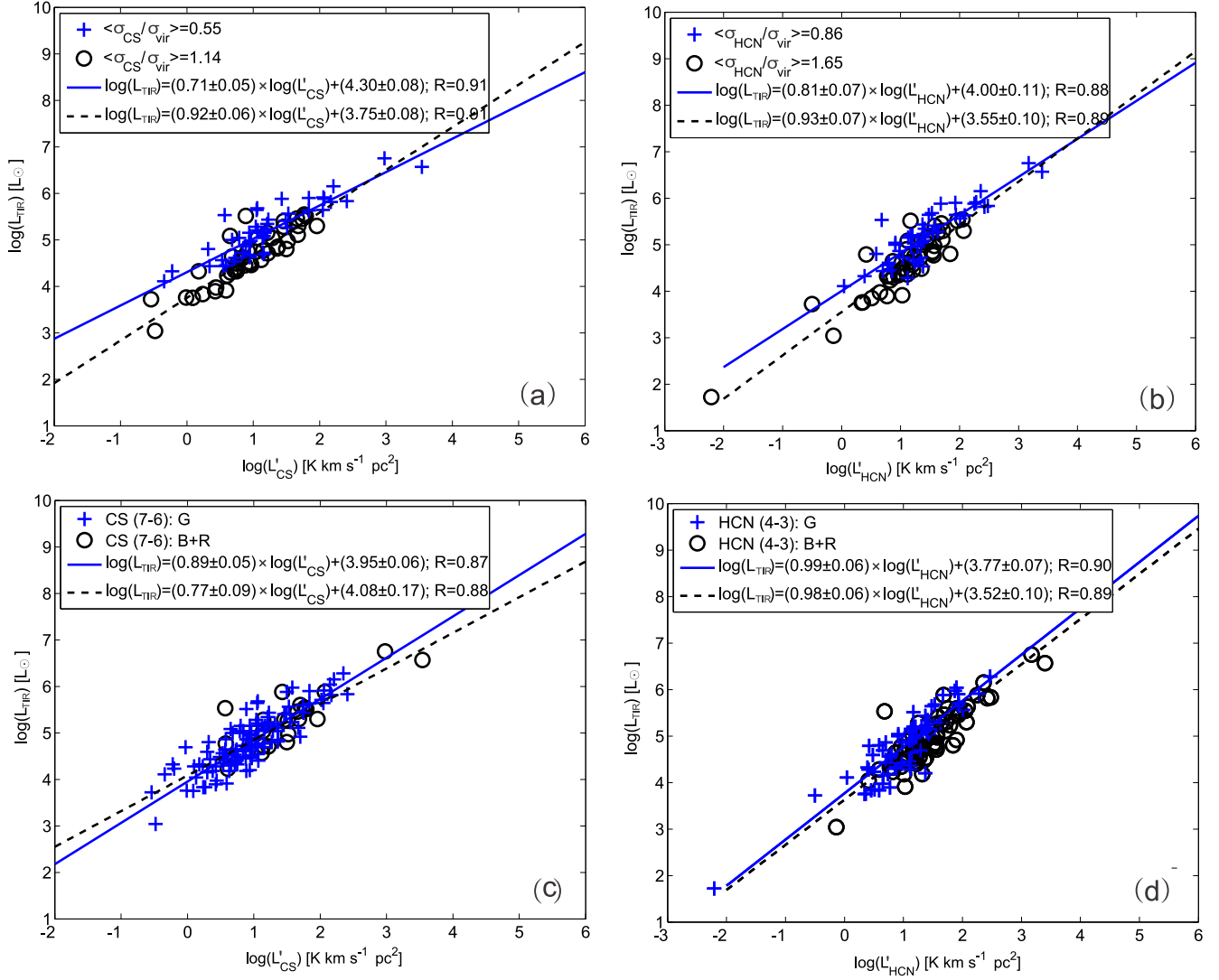
Figure 9. (a): L_{\text{TIR}}-L'_{\text{CS}} correlations for clumps with smallest \sigma_{\text{CS}}/\sigma_{\text{vir}} (blue crosses) and for clumps with largest \sigma_{\text{CS}}/\sigma_{\text{vir}} (open circles). (b): L_{\text{TIR}}-L'_{\text{HCN}} correlations for clumps with smallest \sigma_{\text{HCN}}/\sigma_{\text{vir}} (blue crosses) and for clumps with largest \sigma_{\text{HCN}}/\sigma_{\text{vir}} (open circles). (c): L_{\text{TIR}}-L'_{\text{CS}} correlations for clumps with symmetric profiles (blue crosses) and for clumps with asymmetric profiles (open circles). (d): L_{\text{TIR}}-L'_{\text{HCN}} correlations for clumps with symmetric profiles (blue crosses) and for clumps with asymmetric profiles (open circles).
