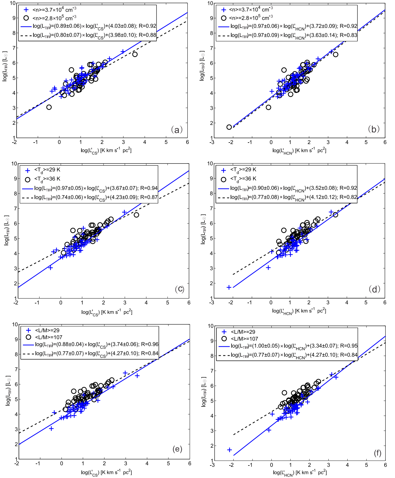
Figure 8. (a) L_{\text{TIR}}-L'_{\text{CS}} correlations for clumps with smallest volume densities (blue crosses) and for clumps with largest volume densities (open circles). (b) L_{\text{TIR}}-L'_{\text{HCN}} correlations for clumps with smallest volume densities (blue crosses) and for clumps with largest volume densities (open circles). (c) L_{\text{TIR}}-L'_{\text{CS}} correlations for clumps with smallest dust temperature (blue crosses) and for clumps with largest dust temperature (open circles). (d) L_{\text{TIR}}-L'_{\text{HCN}} correlations for clumps with smallest dust temperature (blue crosses) and for clumps with largest dust temperature (open circles). (e) L_{\text{TIR}}-L'_{\text{CS}} correlations for clumps with smallest luminosity-to-mass ratios (blue crosses) and for clumps with largest luminosity-to-mass ratios (open circles). (f) L_{\text{TIR}}-L'_{\text{HCN}} correlations for clumps with smallest luminosity-to-mass ratios (blue crosses) and for clumps with largest luminosity-to-mass ratios (open circles).
