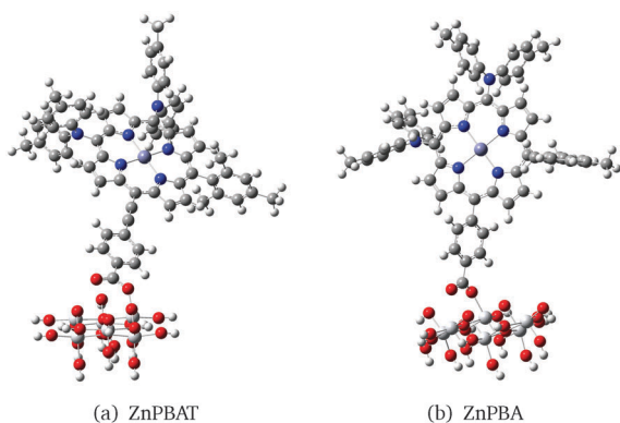
Fig. 3 Optimized geometry for the ZnPBAT and ZnPBA chromophores bound to a TiO 2 cluster.
