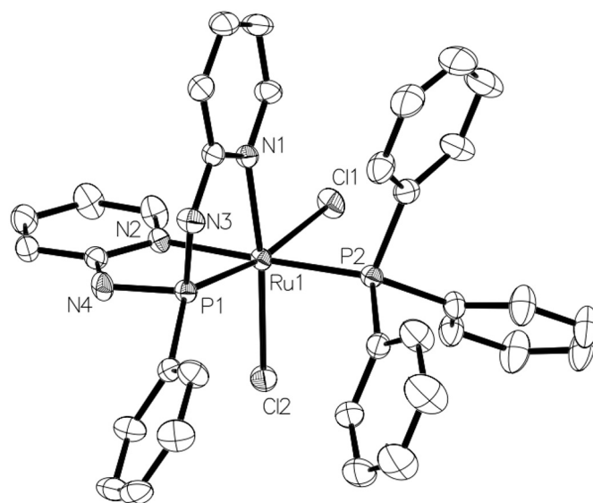
Fig. 1. Crystal structure for complex 1.
