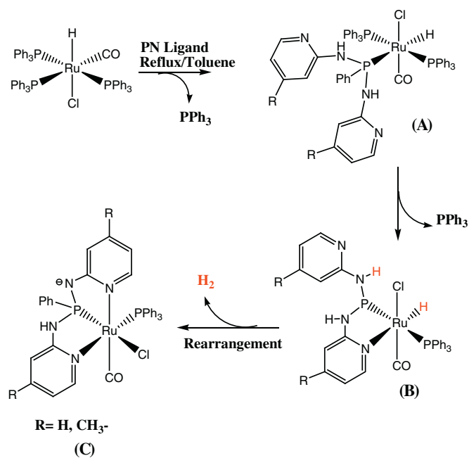
Scheme 2. Likely mechanism for the dehydrogenation of Ru(Cl)(CO)(H)(PPh 3 ) 3 complex containing pincer-type ligands.
