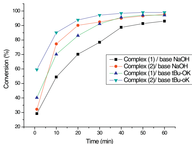
Fig. 2. Catalytic activities of complexes RuCl 2 PPh 3 (PPh(NHPy) 2 ) (1) and [RuCl 2 PPh 3 (PPh(NHPyMe) 2 )] (2) in the transfer hydrogenation of N -benzylideneaniline using different bases. Temperature 50 °C; substrate/catalyst ratio: 100/1.
