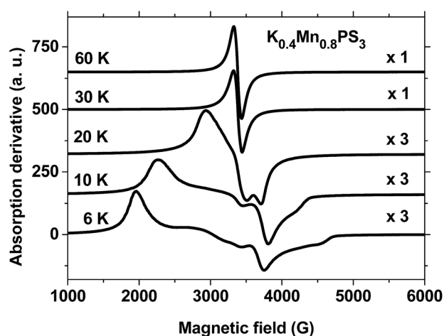
Fig. 4 EPR spectra of the \text{K}_{0.4}\text{Mn}_{0.8}\text{PS}_3 \cdot \text{H}_2\text{O} phase at selected temperatures. Temperatures are indicated on the left and plot magnifications on the right. Microwave frequencies: 9.489 GHz (6–30 K) and 9.471 GHz (60 K).
