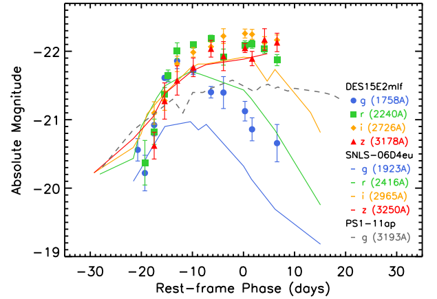
Figure 5. Absolute-magnitude light curves of DES15E2mlf (solid symbols), the z = 1.588 SLSN-I SNLS-06D4eu (solid lines; Howell et al. 2013) and the z = 0.524 SLSN-I PS1-11ap (dashed lines; McCrum et al. 2014). The griz bands are labelled with their rest-frame effective wavelength for each SN.
