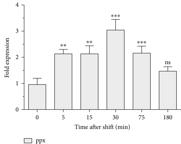
FIGURE 4: Transcriptional levels of ppx gene increase significantly in M. sedula DSM 5348 T cells after a copper shift. Relative transcriptional levels of ppx in M. sedula cells exposed to an 8mM copper shift were measured by qRT-PCR. (** P < 0.01 ; *** P < 0.001 ; ns: nonsignificant).
