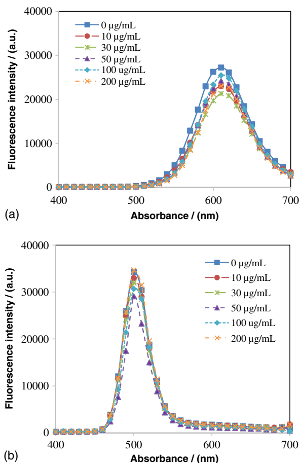
Fig. 5. Effect of arsenic on the fluorescence of biomimetic Cd-based nanoparticles
