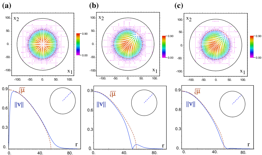
Fig. 1 a The standard vortex described in Theorem 1.2 (iii), b the standard vortex near the boundary of the set \mu > 0 and c the shadow vortex described in Theorem 1.2 (ii) in case a = o(\epsilon |\ln \epsilon|) . The upper panel shows the global minimizer v = (v_1, v_2) as a vector field in \mathbb{R}^2 . In the lower panel, a radial section of |v| taken at the angle \theta indicated in the upper right corner and compared with the Thomas–Fermi limit \sqrt{\mu^+} . Numerical simulations were performed after rescaling the original spatial variable x \mapsto x/\epsilon
