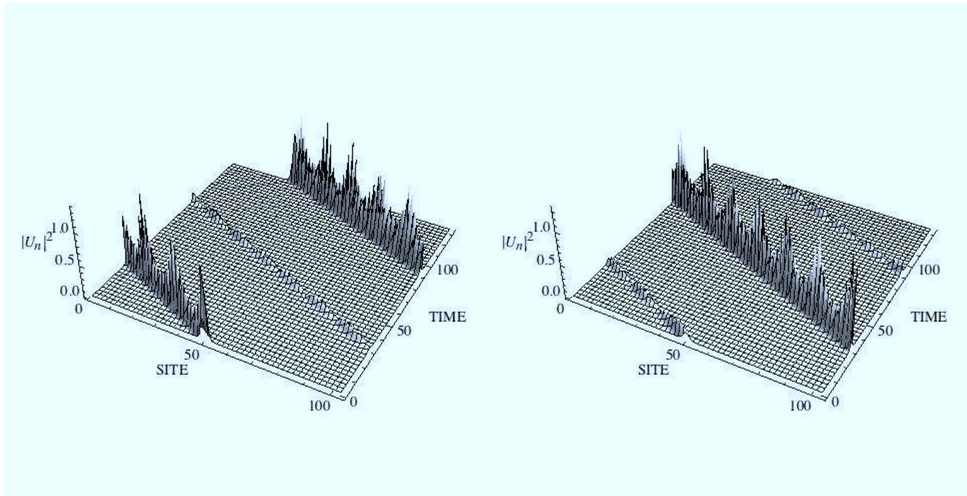
FIG. 7. Möbius case. Time evolution of u_n(z) (left) and v_n(z) (right) for an initial AL soliton on a Möbius strip, for transversal coupling t' = 0.26 . ( \alpha = 1, \beta = 0.5, N = 103 ).
