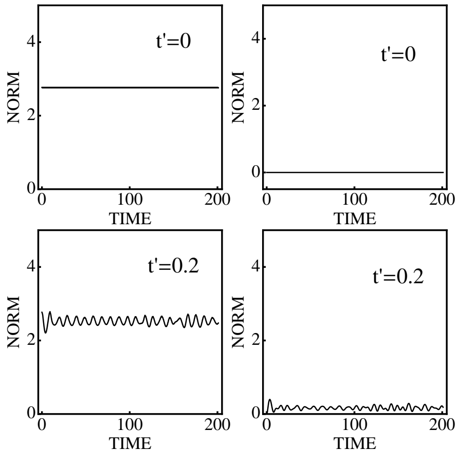
FIG. 2. Untwisted case. Soliton norm of the AL soliton on chain A (left column) and on chain B (right column), for two values of interchain coupling. ( \alpha = 1, \beta = 0.5, N = 103 )
