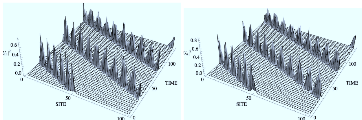
FIG. 8. Möbius case. Time evolution of u_n(z) (left) and v_n(z) (right) for an initial AL soliton on a Möbius strip, for transversal coupling t' = 0.5 . ( \alpha = 1, \beta = 0.5, N = 103 )
