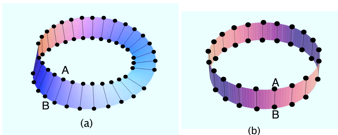
FIG. 1. Geometry of the two ribbons considered in this work: (a) Möbius and (b) Untwisted
