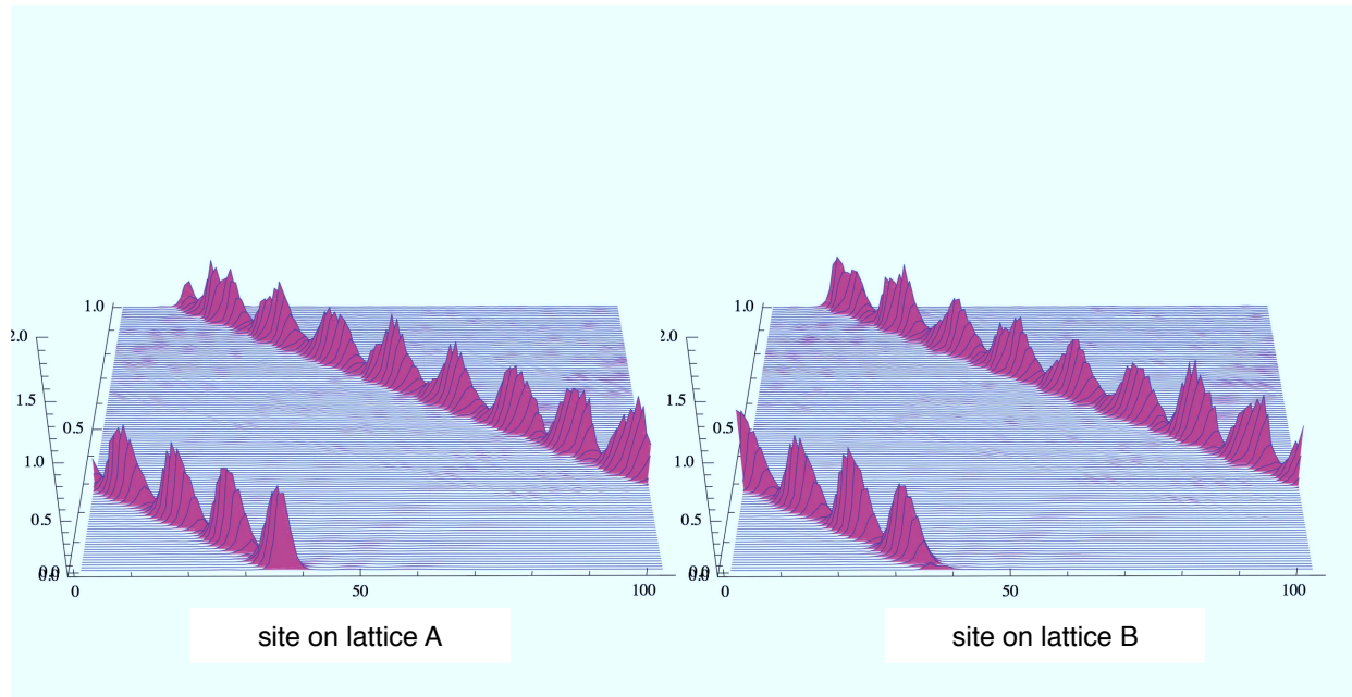
FIG. 4. Untwisted case. Time evolution of u_n(z) (left) and v_n(z) (right) for an initial AL soliton for a normal untwisted strip, and for a transverse coupling value t' = 0.5 ( \alpha = 1, \beta = 0.5, N = 103 )
