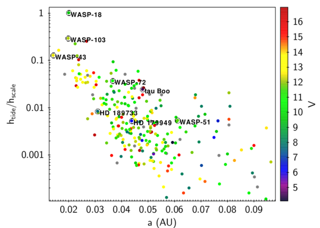
Figure 8. SPI interaction strength proxies for planets with M_p \sin i = 0.1\text{--}13 M_J and a < 0.1 au. The visual magnitude is shown as a guide to the observability of the systems. Planets observed in this study and key systems from the literature are labelled. A null-result for SPI in the particularly extreme WASP-18 system was found by Miller et al. (2012), and attributed to the very low intrinsic activity level of this F6V star; see X-ray non-detection in Pillitteri et al. (2014). Evidence for weak SPI effects have been reported for HD 179949 (Shkolnik, Walker & Bohlender 2003), HD 189733 (Poppenhaeger & Wolk 2014) and tau Boo (Walker et al. 2008).
