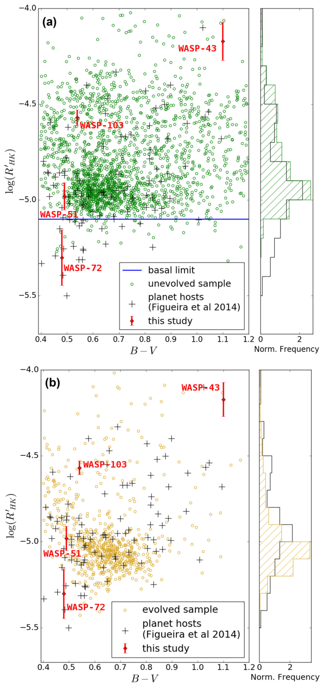
Figure 5. \log(R'_{\text{HK}}) distribution for field stars compared to archival data on planet hosts and our measurements, using (a) unevolved, main-sequence (MS) stars less than 0.45 mag above the average MS and (b) evolved field stars between 0.45 and 2 mag above the average MS. Note that bimodality in the distributions is expected (e.g. Wright 2004; Gray et al. 2006).
