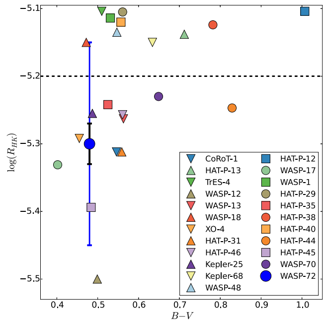
Figure 6. Short-period planet hosts from Figueira et al. (2014) with \log(R'_{\text{HK}}) below the MS basal limit ( -5.1 ) and our measurement of WASP-72. For reference, we show the uncertainty with (blue) and without (black) the uncertainty in our calibration to the Mount Wilson system (equation 2). Stars with |\gamma - V_{\text{ISM}}| < 15 \text{ km s}^{-1} (triangles) may be depressed below \log(R'_{\text{HK}}) = -5.2 by ISM absorption.
