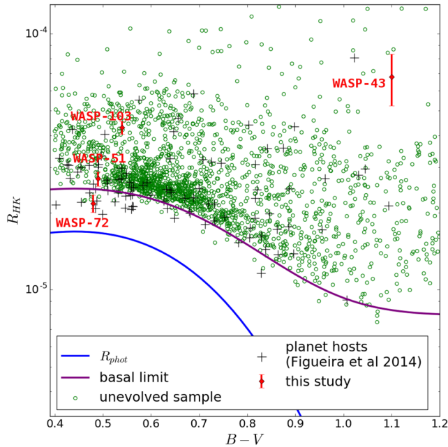
Figure 7. R_{\text{HK}} distribution for unevolved field stars and planet hosts, compared to the chromospheric basal limit and R_{\text{phot}} , the photospheric contribution to R_{\text{HK}} .
