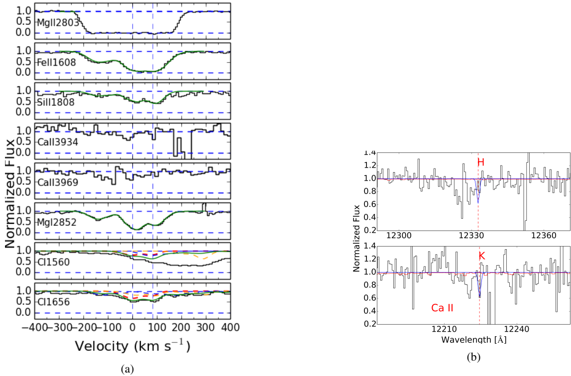
Fig. A.4: J0917+0154 – Same as A.1.
