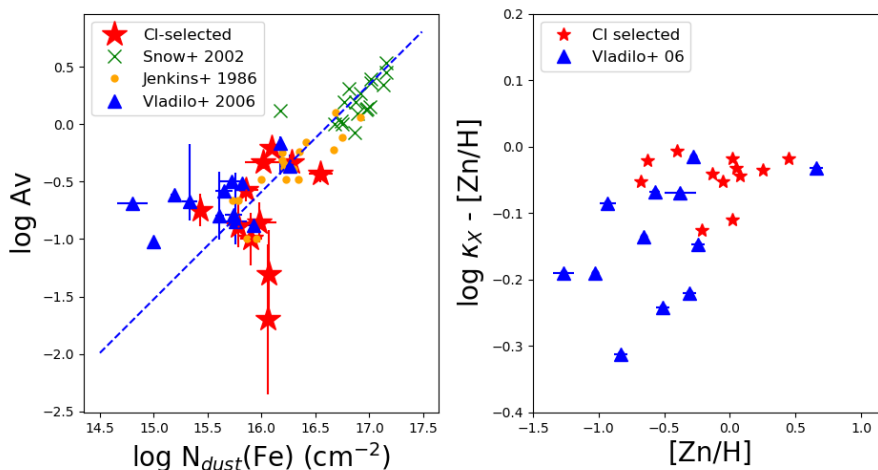
Fig. 8: Left panel: Attenuation A_V versus the Fe II column density into dust. Red stars are for the C I-selected sample, blue triangles correspond to the data from Vladilo et al. (2006), green crosses and orange points are for samples of local interstellar clouds from Snow et al. (2002) and Jenkins et al. (1986), respectively. The blue dashed line is a linear regression of the Milky Way (MW) data with fixed unit slope (see Vladilo et al. 2006). Right panel: The dust-to-gas ratio minus metallicity is plotted against metallicity.
