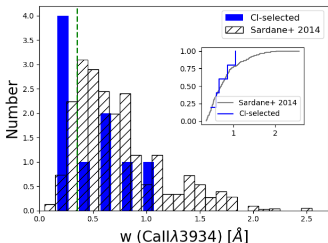
Fig. 6: Blue histogram is the rest equivalent width distribution of the Ca II K lines detected in our sample; grey-hashed histogram is the scaled equivalent width distribution of Ca II K lines detected in the SDSS by Sardane et al. (2014). The two cumulative distributions are shown in the insert; considering the detection limit of SDSS, we applied the Kolmogorov–Smirnov test when W(\text{Ca II } \lambda 3934) > 0.35 \text{ \AA} .
