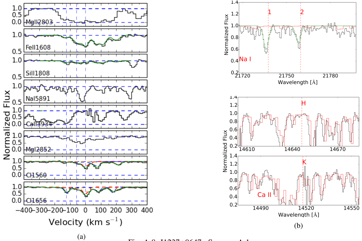
Fig. A.8: J1237+0647 : Same as A.1.
