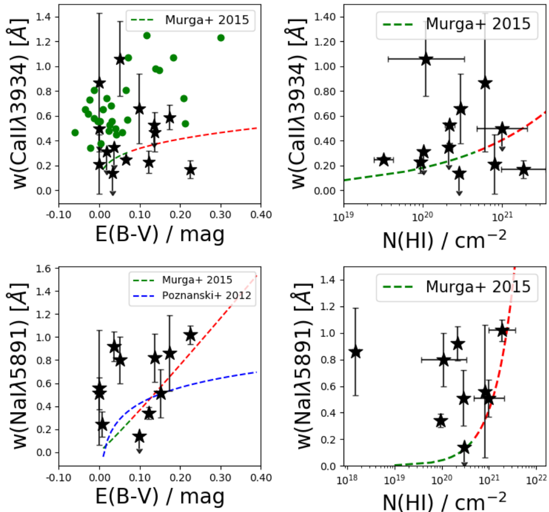
Fig. 9: Left panels: W(\text{Ca II } \lambda 3934) in the upper panel and W(\text{Na I } \lambda 5891) in the lower panel as a function of the colour excess E(B - V) . The green dots are the data from Wild & Hewett (2005). In all panels the green dashed lines correspond to the observations of Murga et al. (2015) in the interstellar and circumgalactic media of the Milky Way. The red dashed lines are extrapolations of these relations. The blue line in the W(\text{Na I}) versus E(B - V) plot is an empirical relation given by Poznanski et al. (2012): \log(E(B - V)) = 2.16 \times W - 1.91 . Right panels: Same as left panels with \log N(\text{H I}) on the x-axis.
