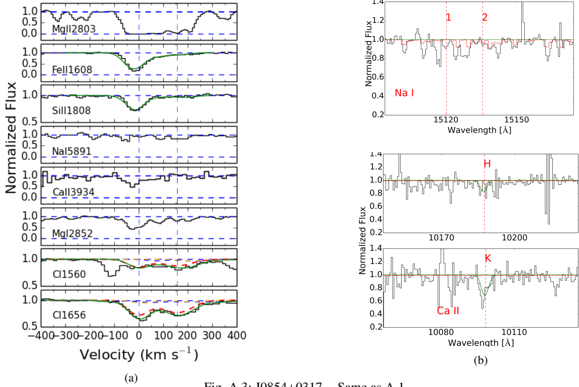
Fig. A.3: J0854+0317 – Same as A.1.
