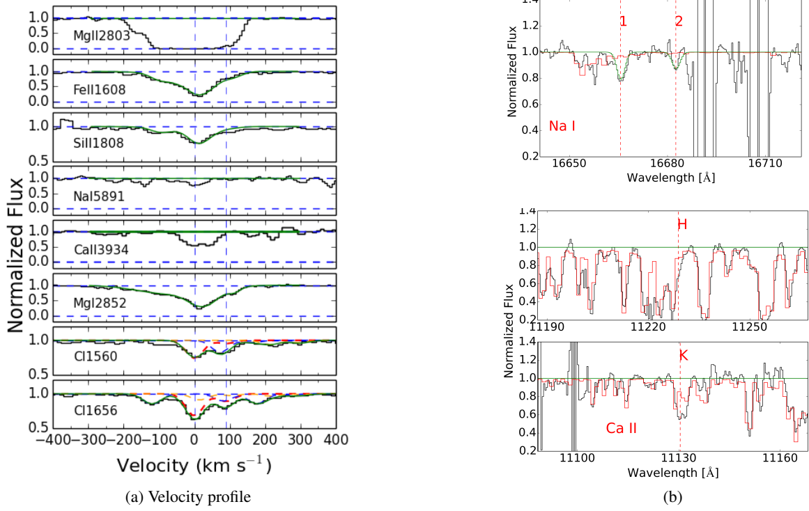
Fig. A.15: J2336-1058 : Same as A.1.
