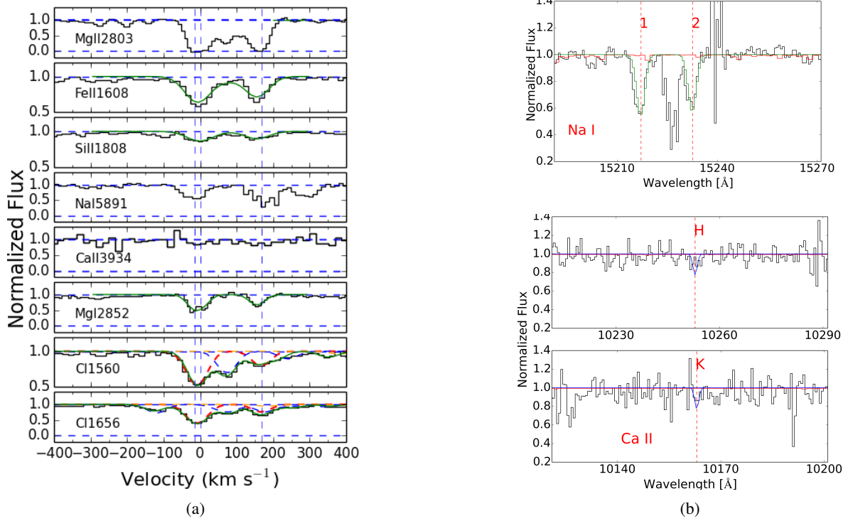
Fig. A.11: J1314+0543 : Same as A.1.
