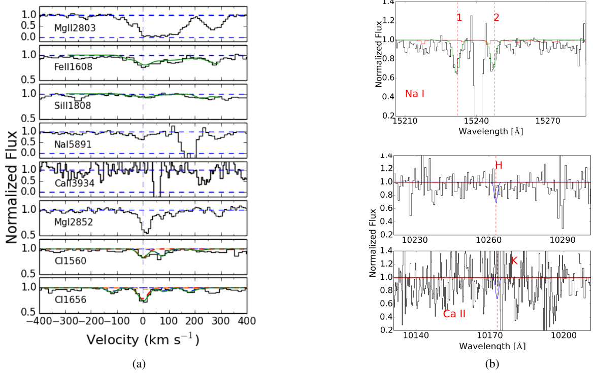
Fig. A.14: J2229+1414 : Same as A.1.
