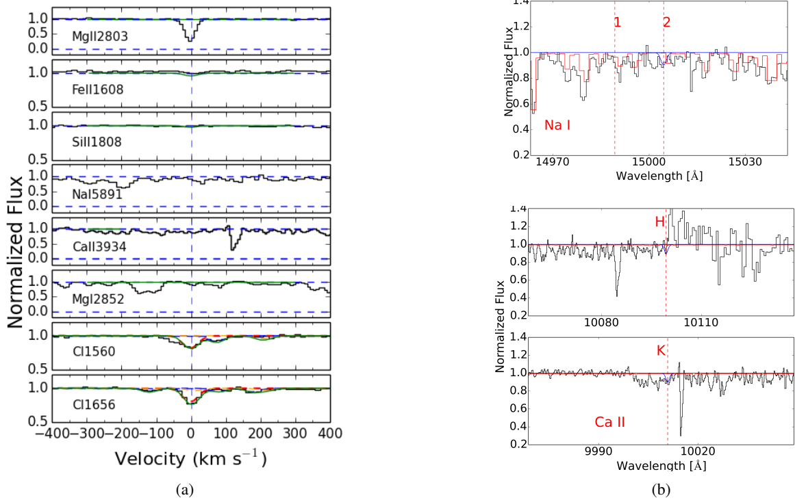
Fig. A.12: J1341+1852 : Same as A.1.
