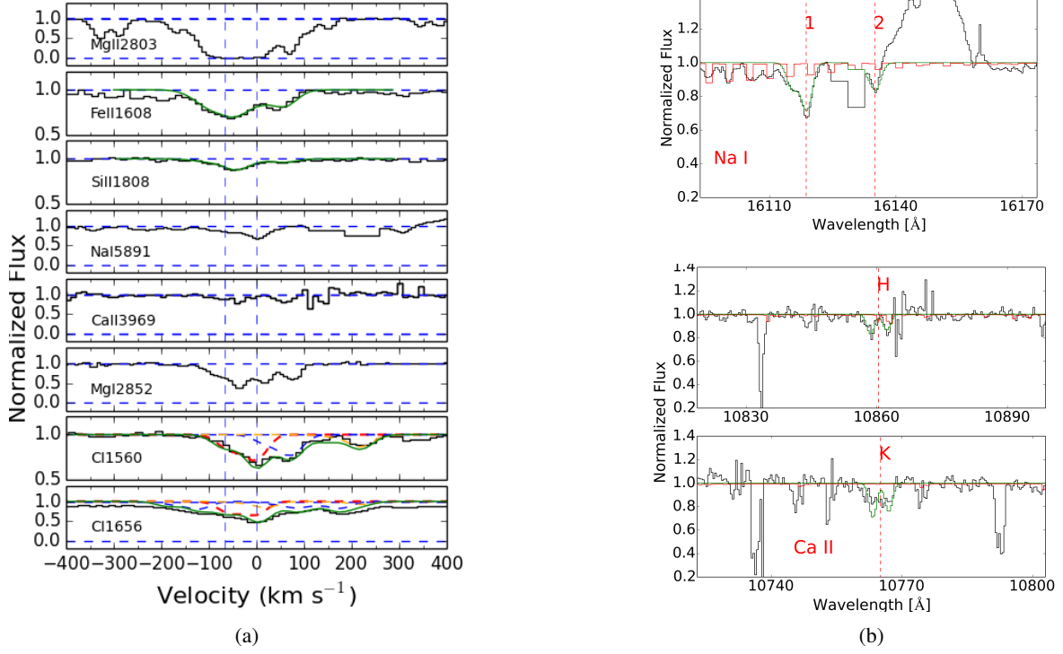
Fig. A.1: J0216-0021 (a) the velocity plot of a sub-set of the absorbing species. The vertical dashed lines indicate the positions of the C I components. Fits to the absorption profiles are over-plotted with the data. For C I transitions, the red dashed line corresponds to the true ground state, the blue dashed line is for the C I* absorption, and the orange dashed line is for the C I** absorption. The redshift is taken in Table 1 to give the zero velocity. Right panels (b): The upper panel is the spectrum at the expected position of Na I \lambda\lambda 5891,5897, the 1 and 2 indicate the Na I \lambda 5891 and Na I \lambda 5897 lines respectively; the lower panel is the spectrum at the expected positions of the Ca I \lambda\lambda 3934,3969 lines, the H and K notations indicate the Ca I \lambda 3969 and Ca I \lambda 3934 lines respectively. The red curve is the telluric spectrum template of X-shooter.
