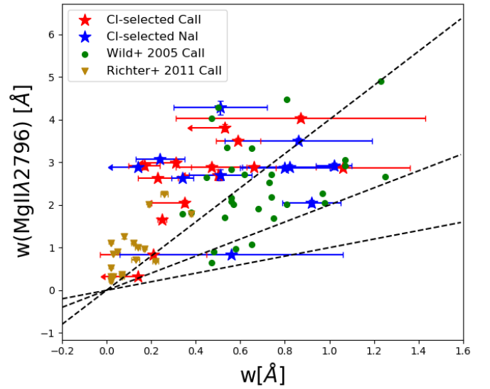
Fig. 13: W(\text{Mg II } \lambda 2796) as a function of Ca II \lambda 3934 (red stars) and Na I \lambda 5891 (blue stars) equivalent widths. Green points are from Wild & Hewett (2005) for systems with 0.6 < z_{\text{abs}} < 1.3 . The orange triangles are the sample from Richter et al. (2011). The three dashed lines are for W(\text{MgII}) / W(\text{CaII}) = 1, 2, \text{ and } 4 respectively.
