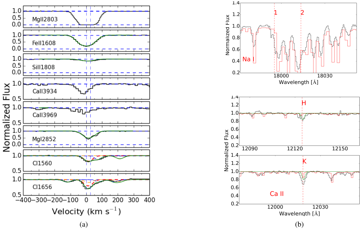
Fig. A.16: J2340-0053 : Same as A.1.
