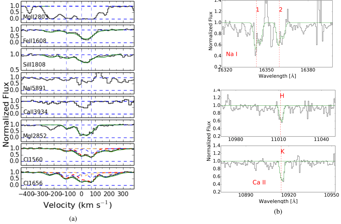
Fig. A.5: J1047+2057 – Same as A.1.
