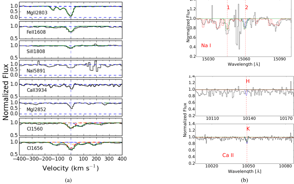
Fig. A.6: J1122+1437 – Same as A.1.
