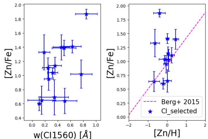
Fig. 2: Left panel: Depletion factor [\text{Zn}/\text{Fe}] versus w(\text{C I } 1560) . Right panel: Depletion factor [\text{Zn}/\text{Fe}] versus metallicity, [\text{Zn}/\text{H}] . The purple dashed line in the right panel is the mean relation observed for typical DLAs (Berg et al. 2015)
