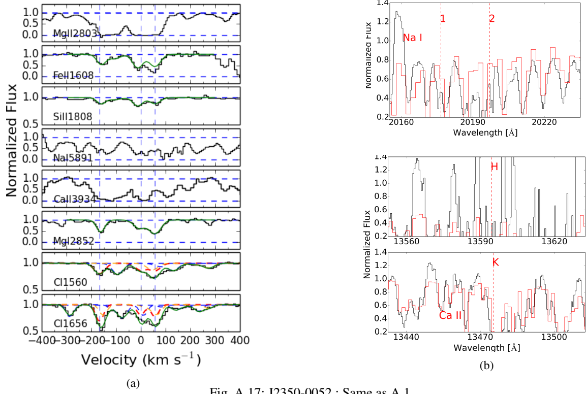
Fig. A.17: J2350-0052 : Same as A.1
