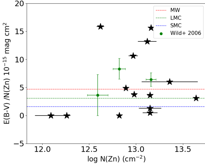
Fig. 10: Dust-to-metal ratio against column density of Zn II. Dashed lines indicate values measured in the MW, LMC, and SMC. Green points correspond to values derived in, respectively, all Ca II systems and sub-samples of high- W value and low- W Ca II systems by Wild et al. (2006).
