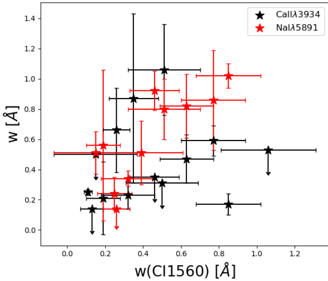
Fig. 11: W(\text{Ca II } \lambda 3934) (black stars) and W(\text{Na I } \lambda 5891) (red stars) as a function of the W(\text{C I } \lambda 1560) .
