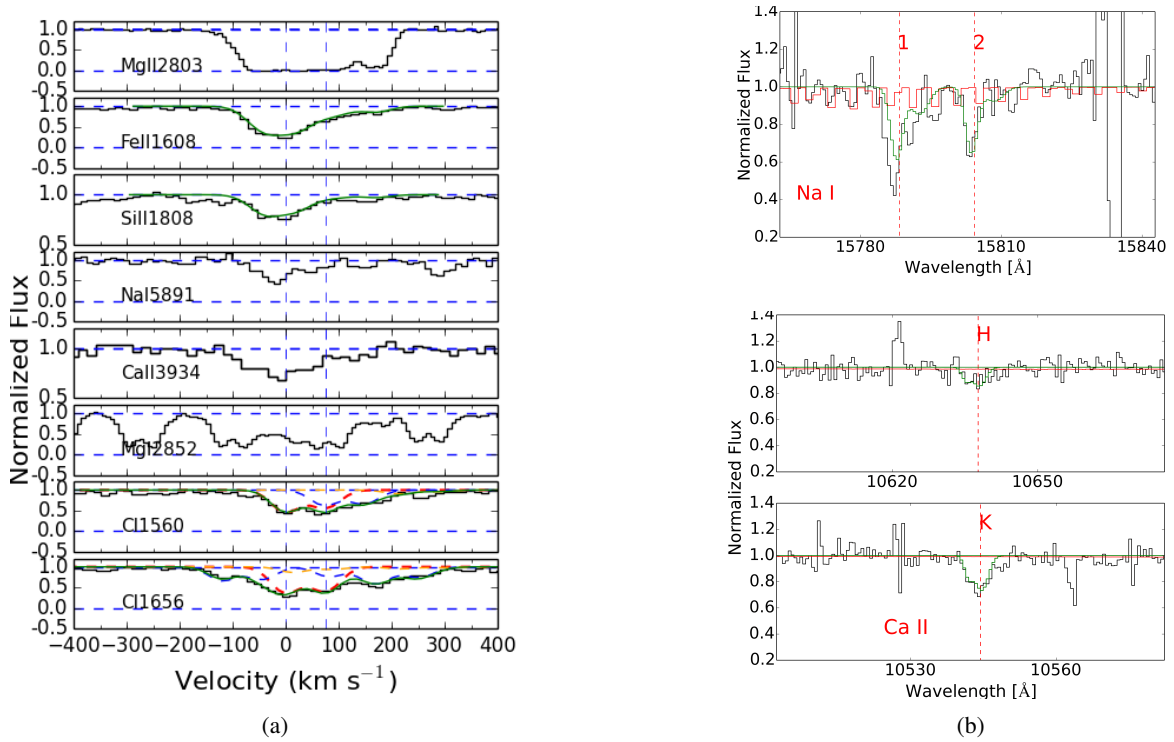
Fig. A.2: J0815+2640 – Same as Fig.A.1
