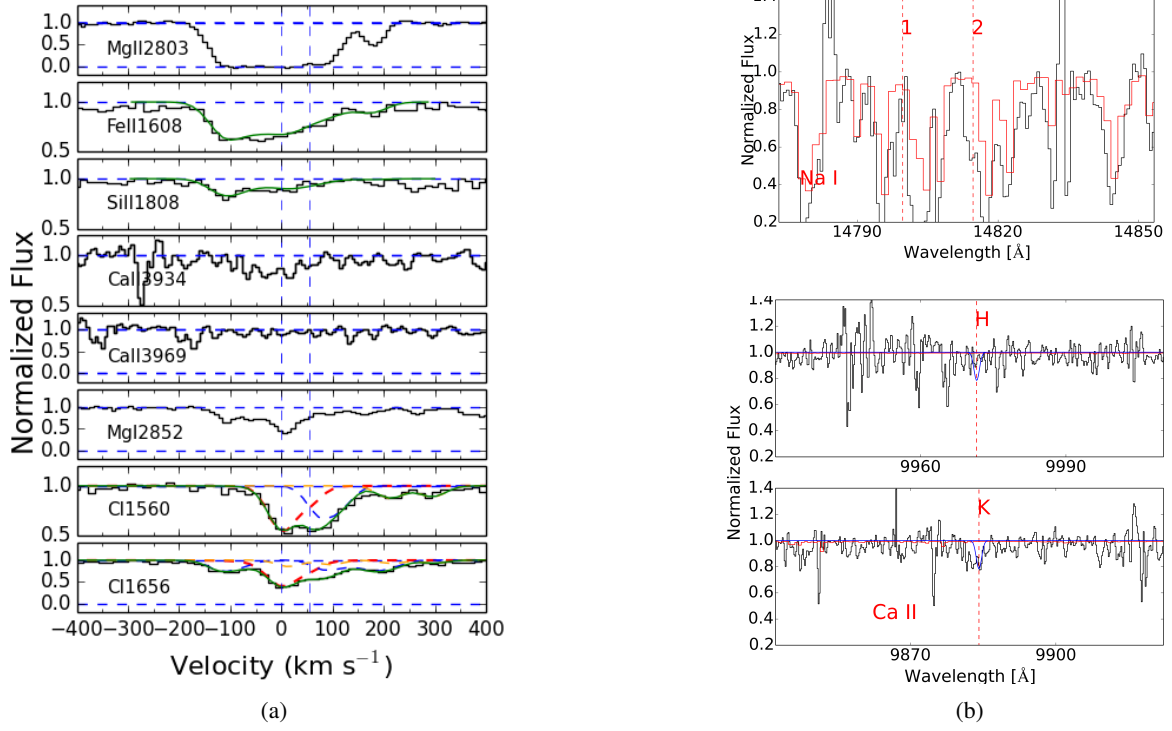
Fig. A.13: J1346+0644 : Same as A.1.
