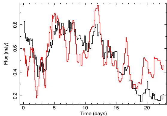
Figure 12. Observed UVW2 light curve (black) with model UVW2 light curve (red) based on a simple disc reprocessing. The normalization of the simulated light curve is arbitrary. The zero-point is the start of the intensive monitoring period.
