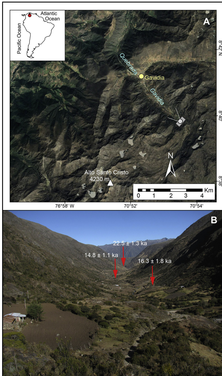
Fig. 15. Glacial landforms between ~3100 and 4200 m a.s.l. in Gavidia Valley in the Mérida Andes. The valley has a U-shaped cross-profile, and has numerous outcrops of striated and polished bedrock (roches moutonnées). Deglaciation happened in two stages: slow retreat between ~22 and 16.5 ka, followed by the complete deglaciation at ~16 ka (Angel et al., 2016). Photo by Eduardo Barreto.
