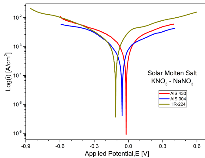
Figure 16. Polarization curves of stainless steel AISI 304, AISI 430, and nickel-based alloy HR-224 in KNaNO 3 (solar salt) at 550 °C and 100 h of exposure.
