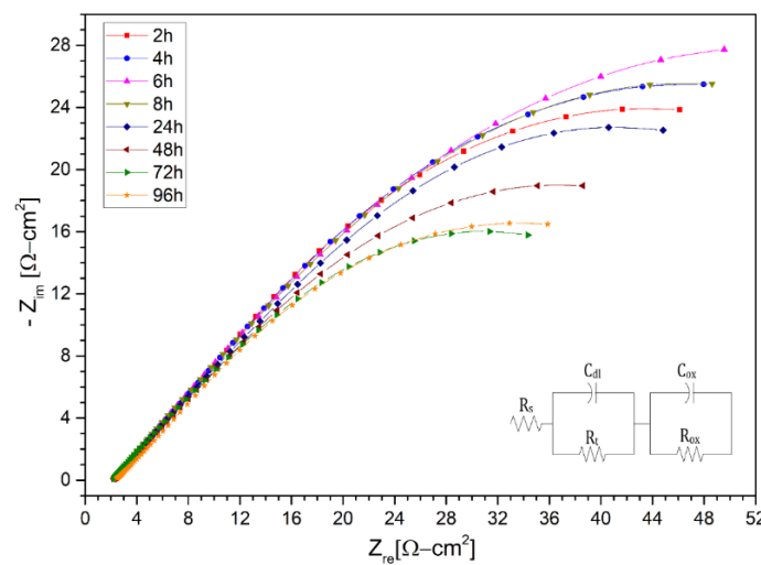
Figure 7. Nysquist diagram of stainless steel 304 layer in (KNa)NO 3 (solar salt) at 2 h, 4 h, 6 h, 8 h, 24 h, 48 h, 72 h and 96 h at 550 °C.
