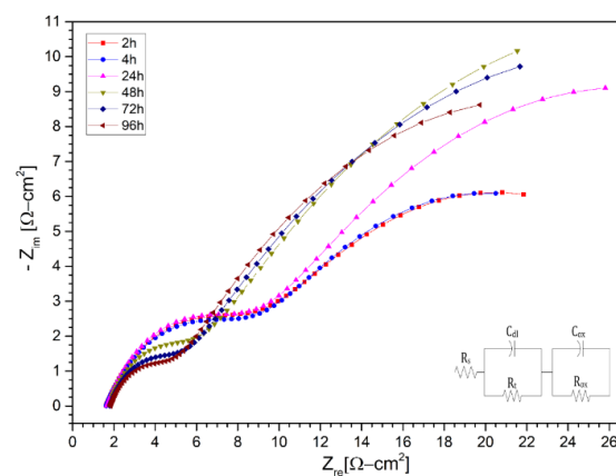
Figure 12. Nysquist diagram of Nickel alloy HR224 layer in (LiNaK)NO 3 (ternary salt with lithium content) at 2 h, 4 h, 24 h, 48 h, 72 h, and 96 h at 550 °C.
