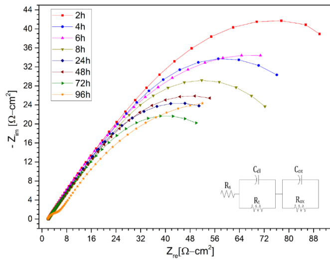
Figure 8. Nysquist diagram of stainless steel 430 layer in (KNa)NO 3 (solar salt) at 2 h, 4 h, 6 h, 8 h, 24 h, 48 h, 72 h and 96 h at 550 °C.
