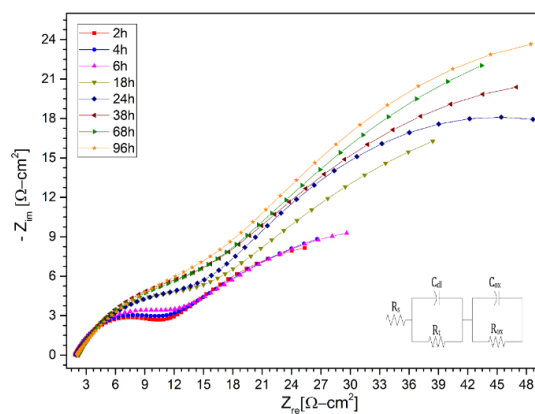
Figure 14. Nysquist diagram of VM12 layer in (LiNaK)NO 3 (ternary salt with lithium content) of 100 h at 2 h, 4 h, 6 h, 18 h, 24 h, 38 h, 68 h, and 96 h at 550 °C.
