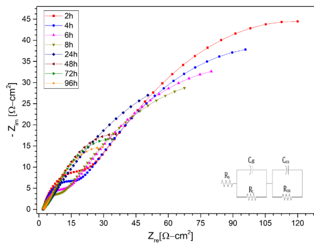
Figure 9. Nysquist diagram of Nickel alloy HR224 layer in (KNa)NO 3 (solar salt) at 2 h, 4 h, 6 h, 8 h, 24 h, 48 h, 72 h and 96 h at 550 °C.
