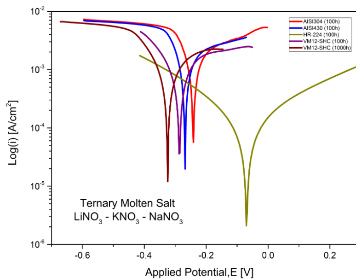
Figure 17. Polarization curves of stainless steel AISI 304, AISI 430, nickel-based alloy HR-224 and ferritic steel VM12 in LiNaKNO 3 (ternary salt with lithium content) at 550 °C and 100 and 1000 h of exposure.
