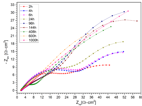
Figure 15. Nysquist diagram of VM12 layer in LiNaKNO 3 (ternary salt with lithium content) of 1000 h at 2 h, 4 h, 6 h, 24 h, 96 h, 144 h, 408 h, 600 h, and 1000 h at 550 °C.
