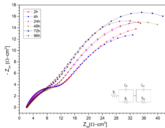
Figure 11. Nysquist diagram of stainless steel 430 layer in (LiNaK)NO 3 (ternary salt with lithium content) at 2 h, 4 h, 24 h, 48 h, 72 h, 96 h at 550 °C.
