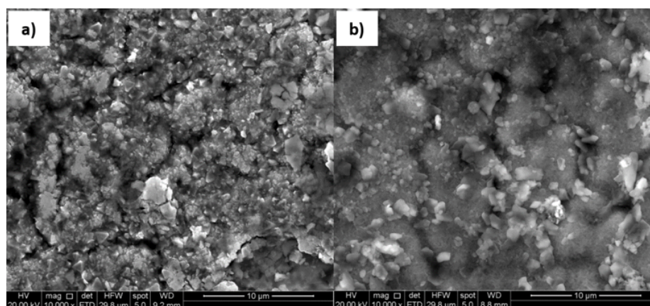
Figure 18. Surface of AISI 304 stainless steel in (a) Solar Salt (b) \text{LiNaKNO}_3 , at 550 °C after 100 h.
