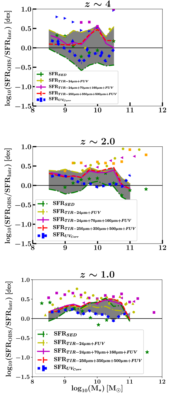
Figure 5. The offset in dex between the various methods used to derive the SFR– M_* relation from the mock EAGLE + SKIRT data with respect the intrinsic EAGLE relation (the solid 0 dex line) at z \simeq 4 (top), z \simeq 2 (medium), and z \simeq 1 (bottom). The dark-green-dashed line represents the offset of the SFR– M_* calculated using the FAST SED fitting code. The orange dash-dotted line represents the SFRs that are inferred from FUV and IR 24 \mu\text{m} luminosities (Wuyts et al. 2008). The magenta solid line represents the results when SFRs are calculated using the 24, 70, and 160 \mu\text{m} luminosities and the relation given by the Dale & Helou (2002) templates. The red-dashed line represents the results when SFRs are calculated using the 250, 350, and 500 \mu\text{m} luminosities and the Dale et al. (2014) templates. The blue-dotted line describes the SFRs derived from UV luminosities dust-corrected using the IRX– \beta relation (Meurer et al. 1999). The grey area describes the offset in dex between the range of methodologies used in this work that spans areas of \sim 0.5\text{--}1 dex at z = 4 , \sim 0.5 dex at z = 2 , and \sim 0.1\text{--}0.5 dex at z = 1 . We see that the level of discrepancy between different methodologies produced by the EAGLE + SKIRT data resembles that of those observed relations reported in the literature.
