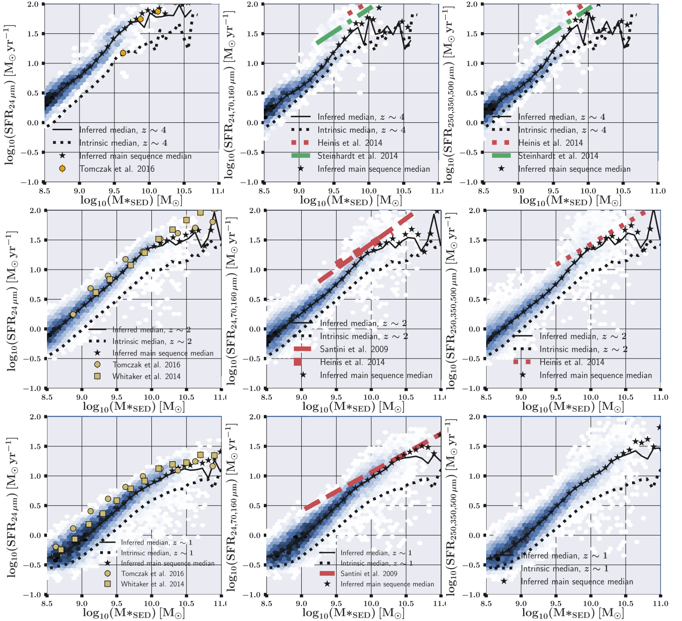
Figure 3. The evolution of the SFR– M_* relation using the EAGLE + SKIRT data using IR wavelengths. The black solid and dotted curves show the median relation inferred from the mock EAGLE + SKIRT observations, while the black dotted line represents the intrinsic relation ( \text{SFR}_{\text{intr}}-M_{*,\text{intr}} ) for the same galaxies. The colour scale indicates the number density of the EAGLE + SKIRT galaxies in the SFR– M_* plane. Different rows show different redshifts. Left-hand panels: SFRs are calculated adopting the luminosity-independent conversion from the observed Spitzer /MIPS 24 \mu\text{m} flux density to the total IR luminosity following (Wuyts et al. 2008). Stellar masses are calculated using the Fitting and Assessment of Synthetic Templates (FAST) code (Kriek et al. 2009). Middle panels: Star formation rates are calculated using the 24, 70, and 160 \mu\text{m} luminosities and their relation with the total IR luminosity given by the Dale & Helou (2002) templates and the TIR–SFR conversion given by Kennicutt & Evans (2012). Right-hand panels: Star formation rates are calculated using the 250, 350, and 500 \mu\text{m} luminosities, the Dale et al. (2014) templates and the conversion given by Kennicutt & Evans (2012). The tension between observed and simulated SFR– M_* relations is generally highly reduced if both SFR and stellar masses are retrieved using similar methods in observations and simulations. In Table 2, we summarize the offset between the intrinsic and inferred relations at different mass bins. The black stars represent the inferred main-sequence relation defined by the exclusion of passive objects with s\text{SFR} < 10^{-9.1} at z \sim 4 , s\text{SFR} < 10^{-9.6} at z \sim 2 , and s\text{SFR} < 10^{-10.1} at z \sim 1 .
