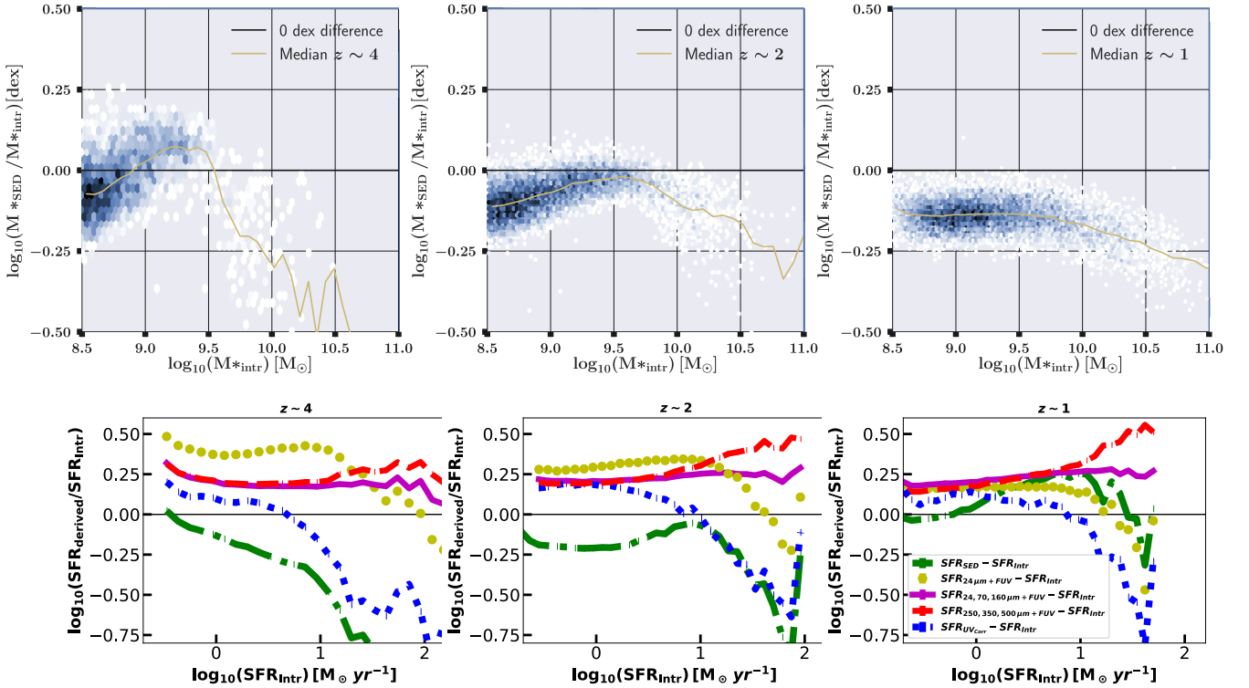
Figure A1. Top panels: Offset in dex between M_{*,SED-FAST} , and M_{*,Intr} . Bottom panels: offset between the SFR_{24,70,160\mu m-r\ Dale\ \&\ Helou\ 2002} , SFR_{SED-FAST} , SFR_{24\mu m-Wuyts\ et\ al.\ 2008} , SFR_{UV+IRX-\beta} , and SFR_{Intr} .
