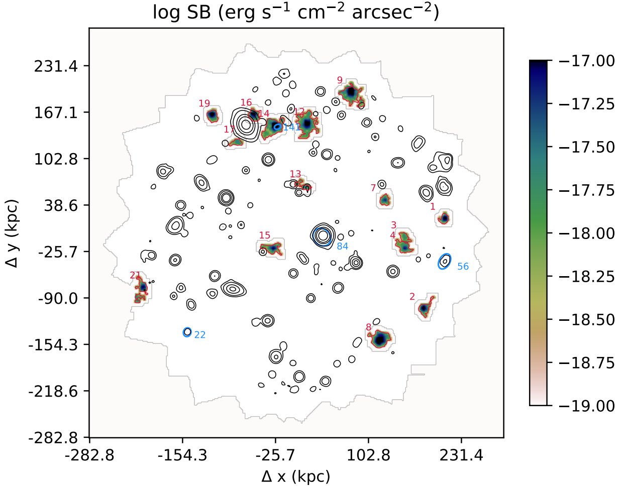
Figure 5. Map of the \text{Ly}\alpha emission detected in the MUSE cube at z > 4 (excluding the quasar itself). Solid contours show continuum emission, whilst the colour scale gives the measured \text{Ly}\alpha surface brightness. Objects detected in \text{Ly}\alpha emission at z > 4 are numbered and outlined in red. Continuum sources at z > 4 are numbered and circled in blue.
