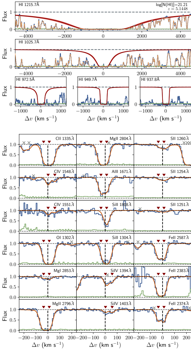
Figure 8. Model fits to the H I absorption and associated metal lines in the X-Shooter spectrum for the DLA system at z = 5.1448 . The data is shown by the blue stepped line in each panel, with the orange curve showing the overall fit within the wavelength range and, in the case of the Lyman series panels, the red curves show the individual strong H I system (with the width of the curves showing the extent given by the best fitting ranges quoted in Table 3). The upright triangles in each metal absorption panel identifies centroids of individual absorption components with the given velocity range of the DLA. The grey crosses indicate absorption features identified as not being at the same redshift (within the given velocity range) of the DLA.
