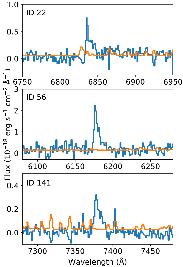
Figure 3. Spectra of all three continuum detected galaxies at z > 4 (excluding the quasar, see also Table 1). At these redshifts, spectroscopic identification is based on Ly \alpha emission which often shows an asymmetric profile.
