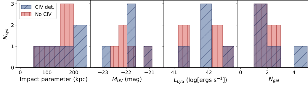
Figure 16. Properties of closest detected galaxies (including both emission and continuum detected) split by whether proximate C IV absorption is detected (blue diagonal hatched histograms) or not detected (red vertical hatched histograms).
