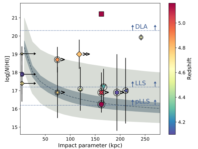
Figure 12. Neutral hydrogen column densities as a function of impact parameter from the nearest detected galaxy within |\Delta v_{-200}| < 1000 \text{ km s}^{-1} . Symbols are consistent with those given in Fig. 11. Absorber-galaxy pairs lying within |\Delta v_{-200}| < 500 \text{ km s}^{-1} are circled. Where multiple galaxies are detected at the same redshift as a given absorber, chevrons are added to the symbol denoting the number of additional galaxies. Limits to the right mark the column density of the absorbers for which we do not identify galaxies. The dashed curve and shaded regions illustrate the median and [32%,68%] and [10%,90%] column density ranges predicted by the EAGLE simulations.
