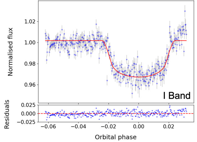
Figure 4. SAAO 1 m/SHOC I-band photometry from the night 2018 December 20 th showing a primary eclipse of NGTS J0930-18 plotted in phase. The red line shows the model fit obtained from joint modelling of photometric and spectroscopic data.
