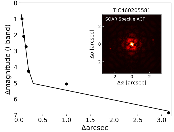
Figure 3. Speckle-imaging of TOI 837. Contrast limits from SOAR HRCam imaging were derived from point-source injection-recovery experiments. Star A ( \Delta T = 4.7 , 2.3'' West) is detected, and is also a resolved Gaia source. It is co-moving with TOI 837, and its parallax and on-sky position imply that it is physically separated from TOI 837 by 6.6 \pm 0.1 pc.
