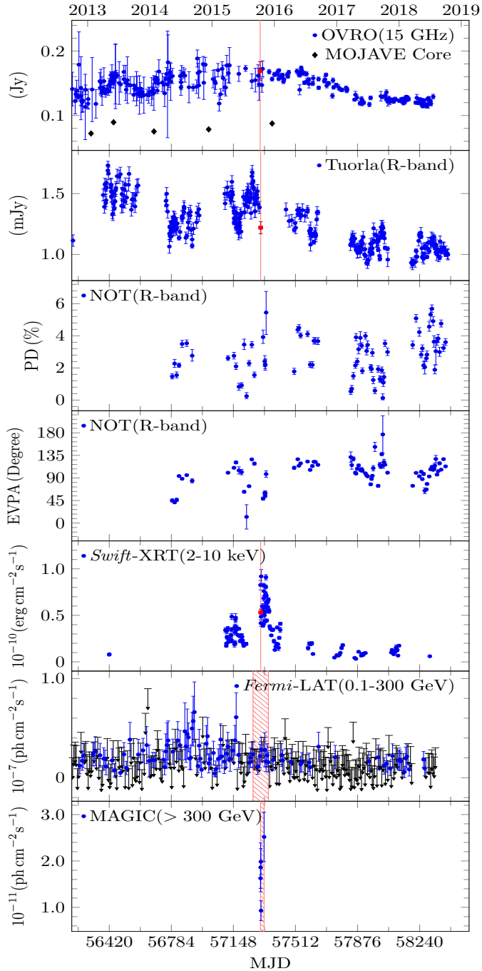
Fig. 3. Same description as in Fig. 1 for IES 1727+502.
