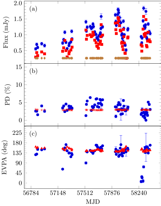
Fig. C.5. Same description as in Fig. C.1 but for 1ES 2344+514.
