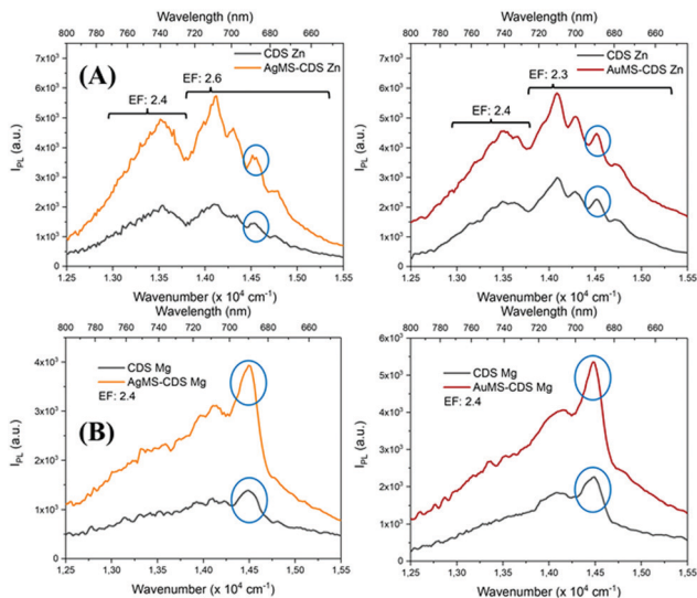
Fig. 8 SEL spectra of (A) ZAO and (B) MAOC on Ag@SiO 2 (orange) and Au@SiO 2 (red) MSs and their counterparts without MSs (black). The blue circle indicates the ZPL.
