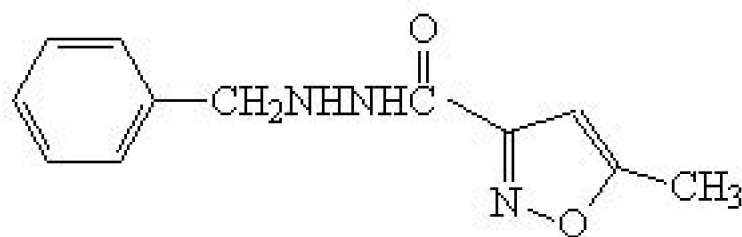
ISOCARBOXAZIDA
