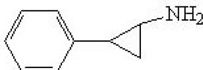
TRANILCIPROMINA
