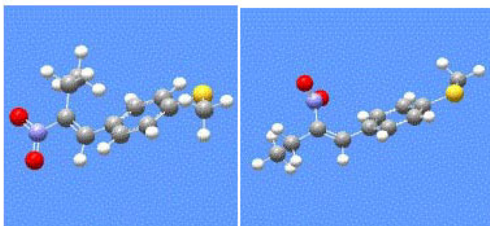
ISOMERO (E)
