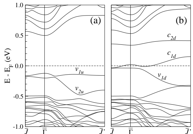
FIG. 4: Electronic band structure for the Fe adatom on the Bi lines at most stable structure. (a) and (b) indicate the majority and minority spin bands, respectively.
