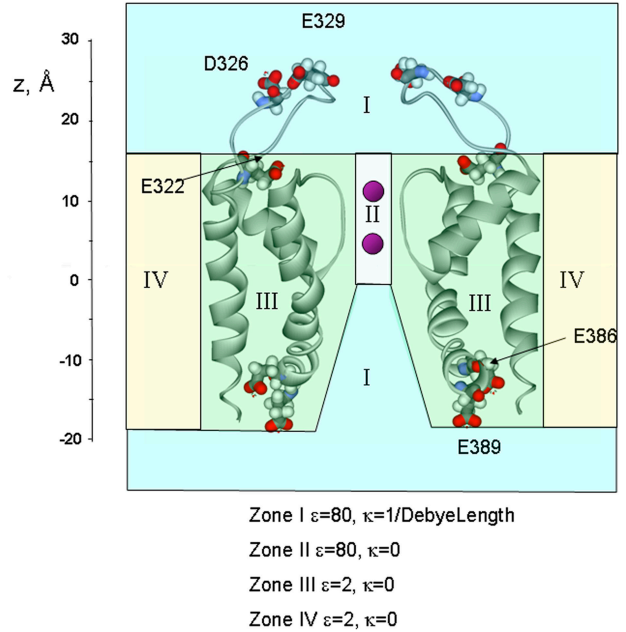
Figure 3. Calculation of the electrostatic potential, \phi(r) by solving the PB equation. In the PB equation \epsilon(r) and \kappa^2(r) are the position-dependent dielectric constant and ionic screening constant, respectively, and \rho(r) is the total atomic charge distribution in the system. \kappa(r) is 0 in zones II, III, and IV, and it is 1/9.8 Å -1 for zone I. Internally located residues E386 and E389 and externally positioned residues E322, D326, and E329 are represented as CPK space-filling mode. In solving the PB equation the bilayer was considered a continuum with a dielectric constant of two, the protein as a continuum with a dielectric constant of two and the solutions a continuum with a dielectric constant of 80.
