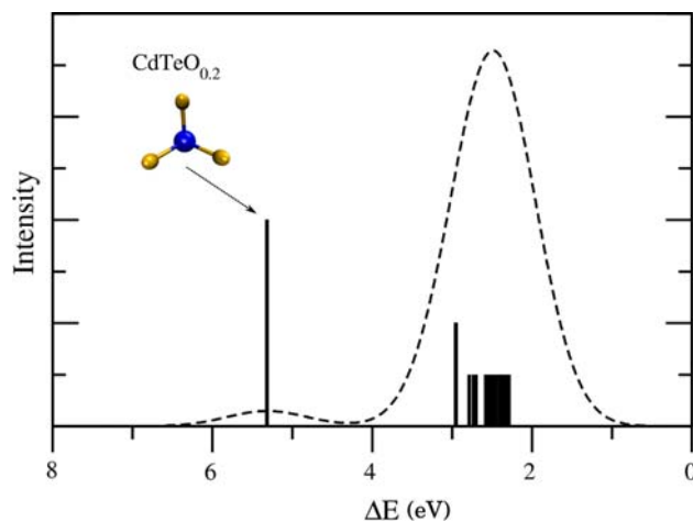
Fig. 2 (Color online) The calculated tellurium XPS spectrum is shown for CdTeO 0.2 . The bars indicate the tellurium energy shifts and the height of the bars denote the number of oxygen neighbors which was calculated within a cutoff radius of 2.32 Å. Typical Te environments are depicted as well, where the blue balls are Te atoms and the yellow ones represent oxygen
