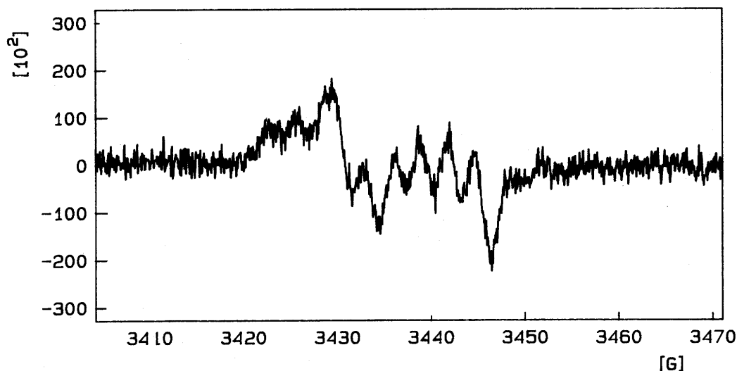
Figure 2: ESR spectra of compound 18 in DMSO.
