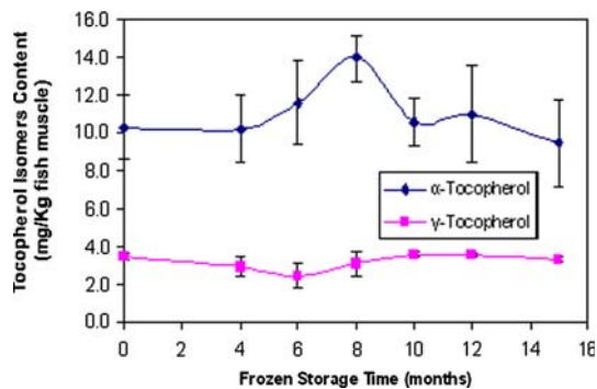
Fig. 3 Tocopherol isomers present during coho salmon frozen storage. Bars denote standard deviations of the mean ( n = 5 ). Starting fresh fish values: 11.0 \pm 0.5 and 3.3 \pm 0.4 for alpha and gamma isomers, respectively
