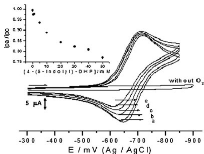
Figure 2. Cyclic voltammograms corresponding to the \text{O}_2/\text{O}_2^{\bullet-} redox couple: (A) \text{O}_2 saturated solution; (B) +1 mM; (C) +10 mM; (D) +30 mM; and (E) +50 mM of 4-(5-indolyl)-DHP. Sweep rate: 0.1 \text{ Vs}^{-1} . Electrolytic media: DMSO + 0.1 M de TBAHFP. Insert: i_{pa}/i_{pc} ratio of \text{O}_2/\text{O}_2^{\bullet-} redox couple in the presence of different concentrations of 4-(3-indolyl)-DHP
