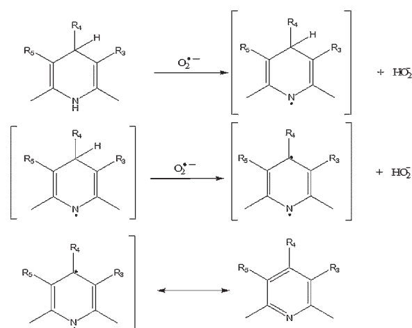
Scheme 1. Proposed mechanism of reaction between C4-indolyl 1,4-dihydropyridines with superoxide anion
