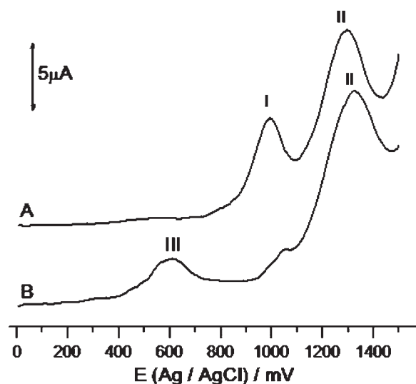
Figure 4. Differential pulse voltammograms of: (A) 1 mM 4-(5-indolyl)-DHP (B) 1 mM 4-(5-indolyl)-DHP + 1.5 mM de KO_2 , DMSO + 0.1 M TBAHFP
