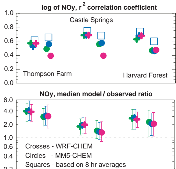
Fig. 4. As in Fig. 3, except for NO_y . Because of log-normal distributions in NO_y concentrations and model errors, Pearson r^2 correlation coefficients are from logarithms of mixing ratios, and biases are represented by median model/observed ratios.
