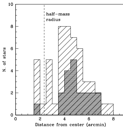
Fig. 2. Radial distribution of the observed stars. The dark shaded area indicates hot stars ( T_{\text{eff}} \geq 20000 K). The half-mass radius from Harris (1996) is also indicated.
