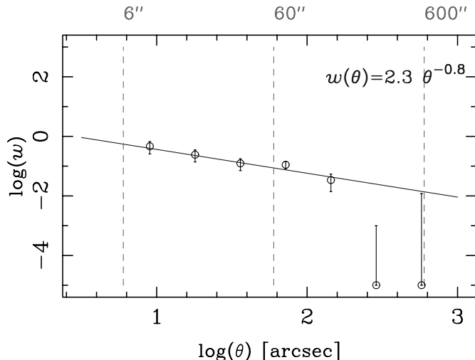
FIG. 19.—Angular autocorrelation function of UVR-selected LBG candidates (open circles with error bars) with fit (solid line) labeled. [See the electronic edition of the Supplement for a color version of this figure.]
