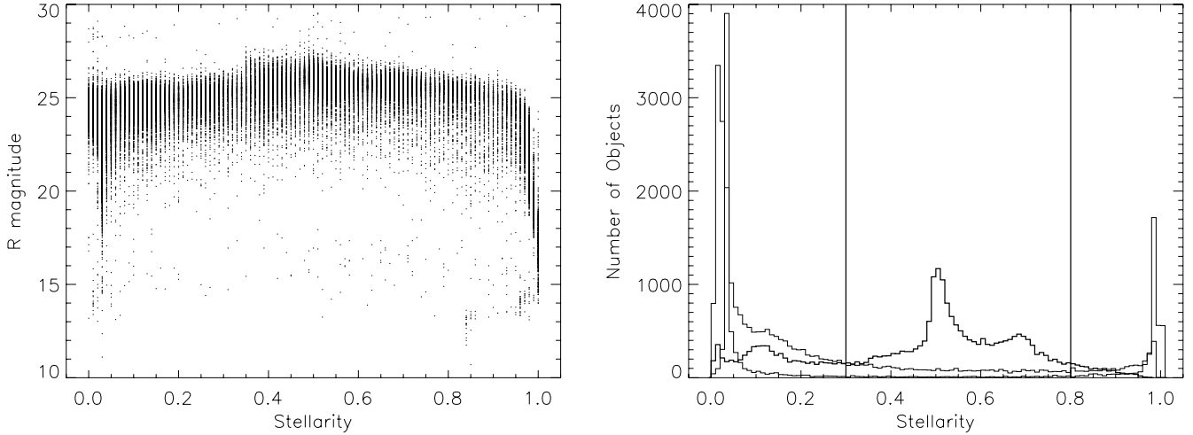
FIG. 13.—SEExtractor stellerity classification for objects in our catalog. The left panel shows stellerity vs. total R -band AB magnitude and reflects confusion for saturated objects at R < 19 . The right panel shows a histogram of stellerity, with vertical solid lines separating galaxies (stellerity \leq 0.3 ), uncertain objects ( 0.3 < \text{stellerity} < 0.8 ), and stars (stellerity \geq 0.8 ). The classification is clean at R < 23 ( light histogram ), shows an increasing fraction of uncertain objects at 23 \leq R < 25 ( medium histogram ), and breaks down at R \geq 25 ( dark histogram ).
