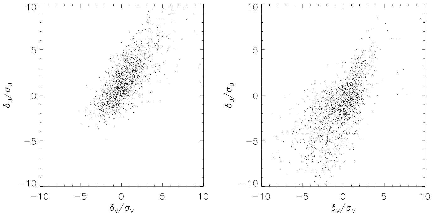
FIG. 11.—Errors in estimated V fluxes divided by reported 1\sigma flux uncertainties in V vs. errors in estimated U fluxes divided by reported 1\sigma flux uncertainties in U for simulated galaxies. The left panel shows results for the AUTO aperture as chosen by SExtractor, and the right panel shows results for the corrected aperture fluxes described in the text.
